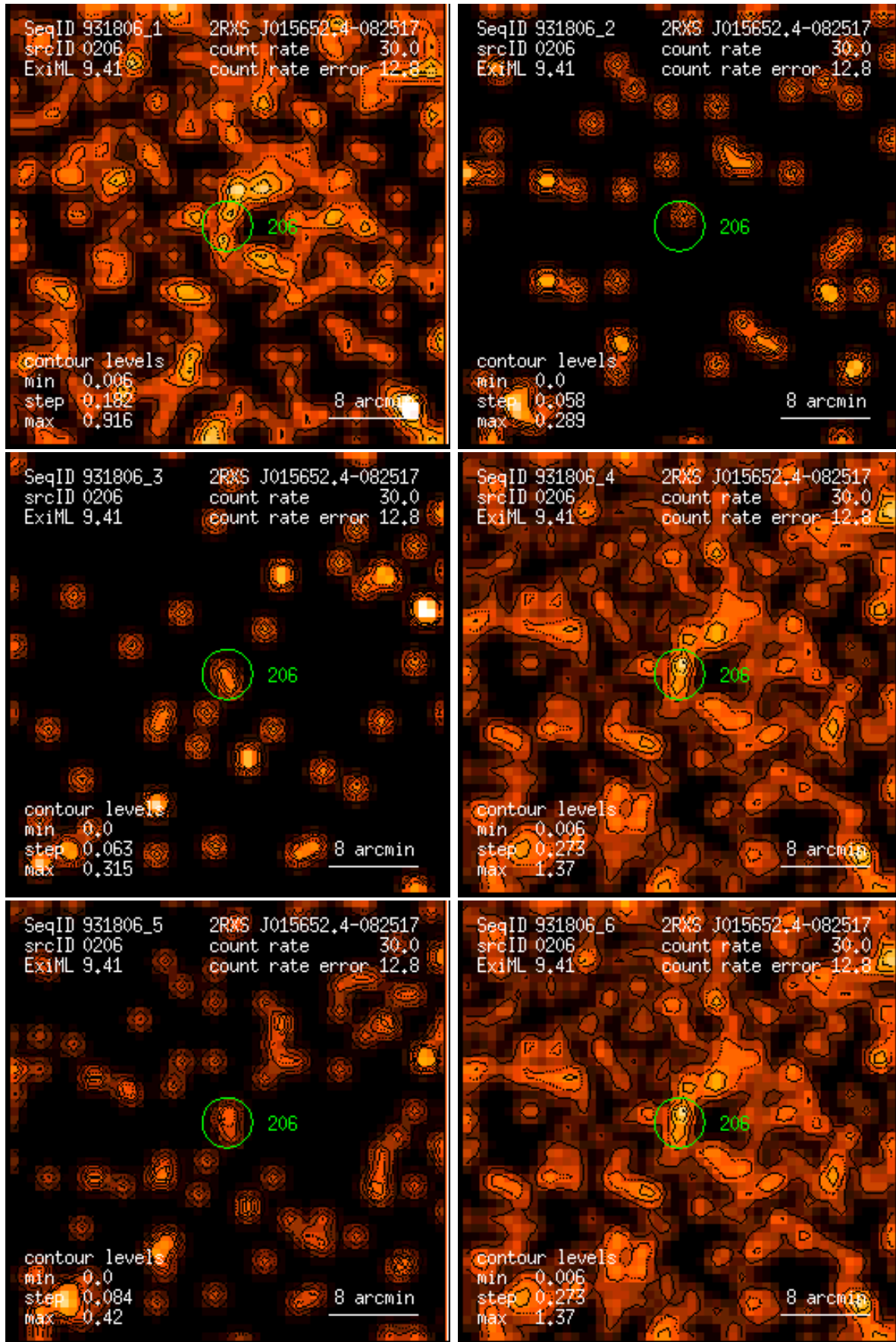
Figure 206: RASS 931806: detection 0206: band rate images, Gaussian filter: (1) PSPC channels 11 – 41, (2) 52 – 90, (3) 91 – 201, (4) 11 – 235, (5) 52 – 201, (6) 11 – 201. Broad band rates in counts/ks. Band rate contour levels in counts/ks/arcmin 2 .
