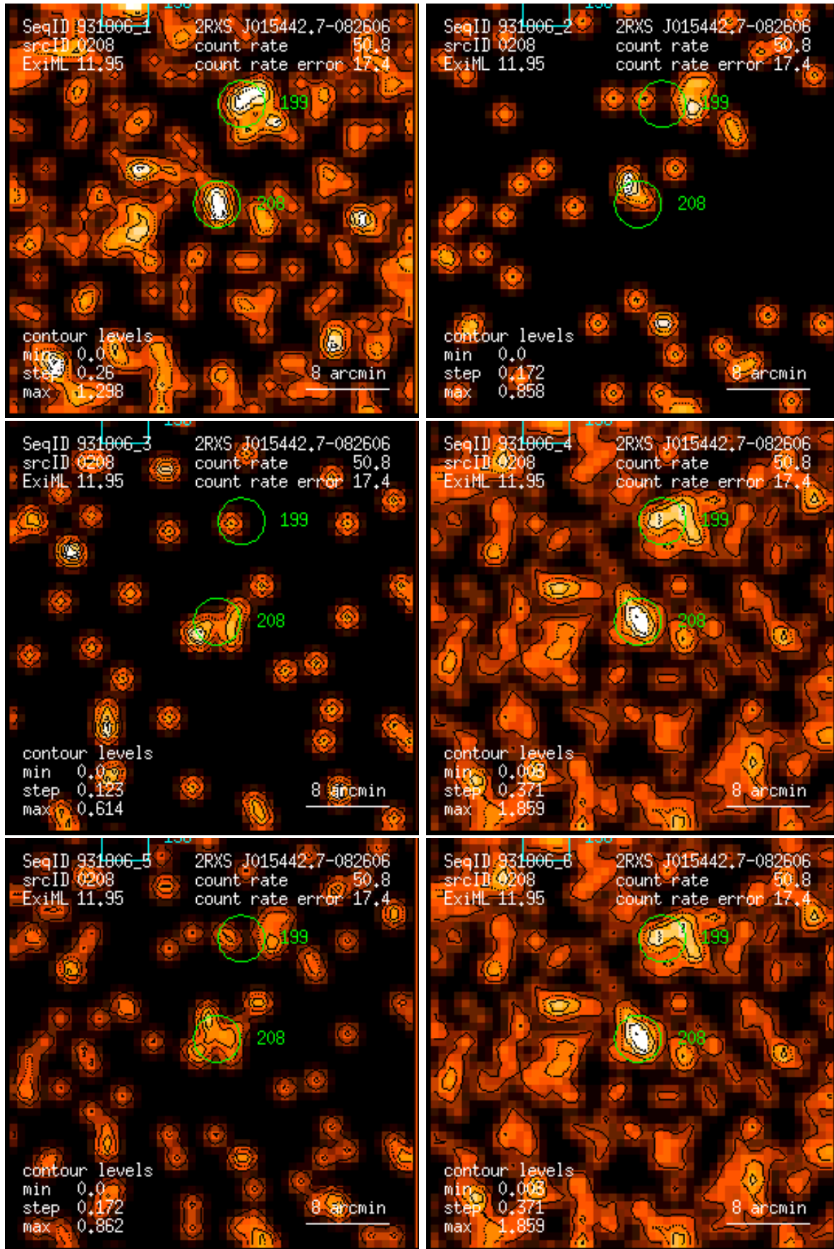
Figure 208: RASS 931806: detection 0208: band rate images, Gaussian filter: (1) PSPC channels 11 – 41, (2) 52 – 90, (3) 91 – 201, (4) 11 – 235, (5) 52 – 201, (6) 11 – 201. Broad band rates in counts/ks. Band rate contour levels in counts/ks/arcmin 2 .
