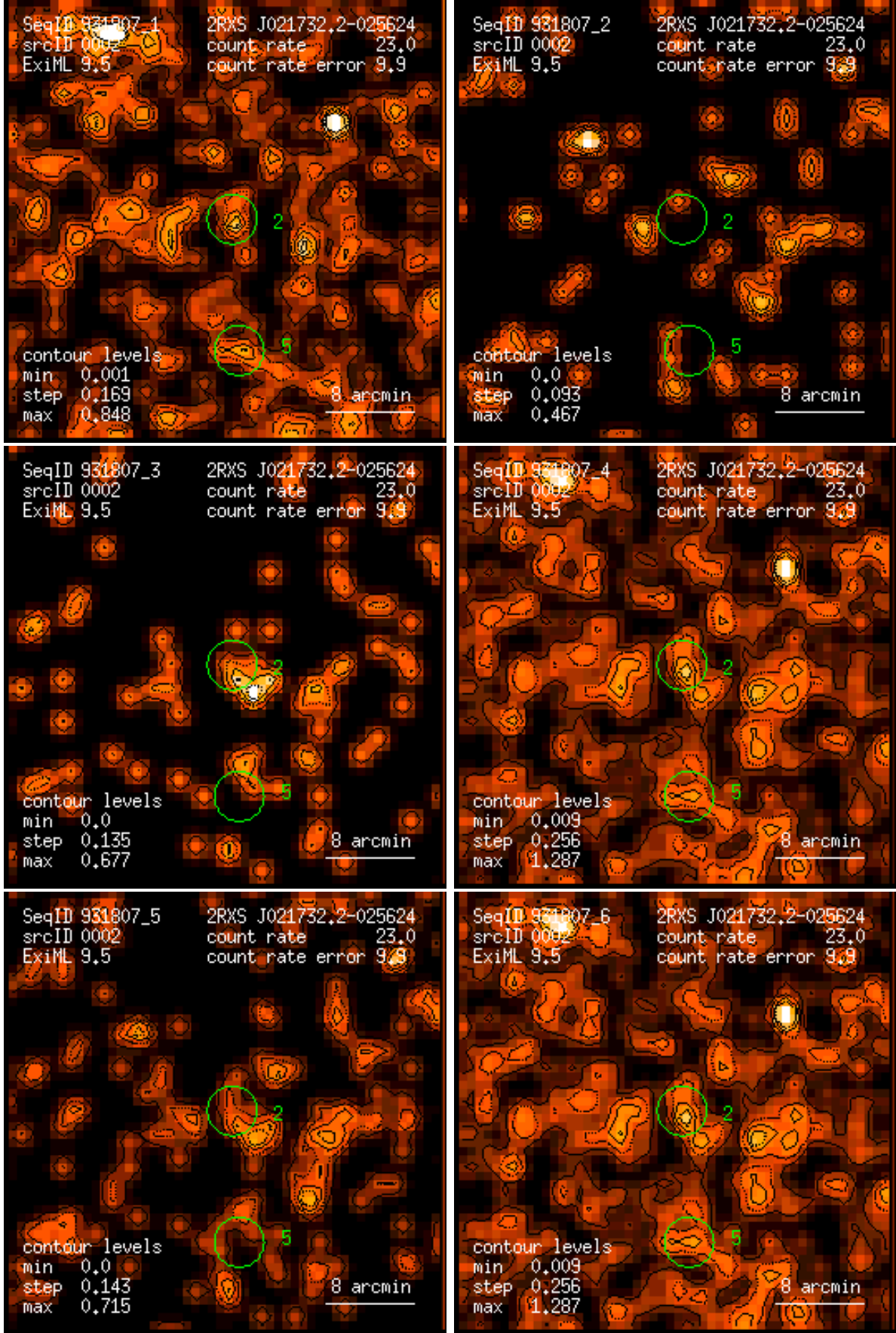
Figure 2: RASS 931807: detection 0002: band rate images, Gaussian filter: (1) PSPC channels 11 – 41, (2) 52 – 90, (3) 91 – 201, (4) 11 – 235, (5) 52 – 201, (6) 11 – 201. Broad band rates in counts/ks. Band rate contour levels in counts/ks/arcmin 2 .
