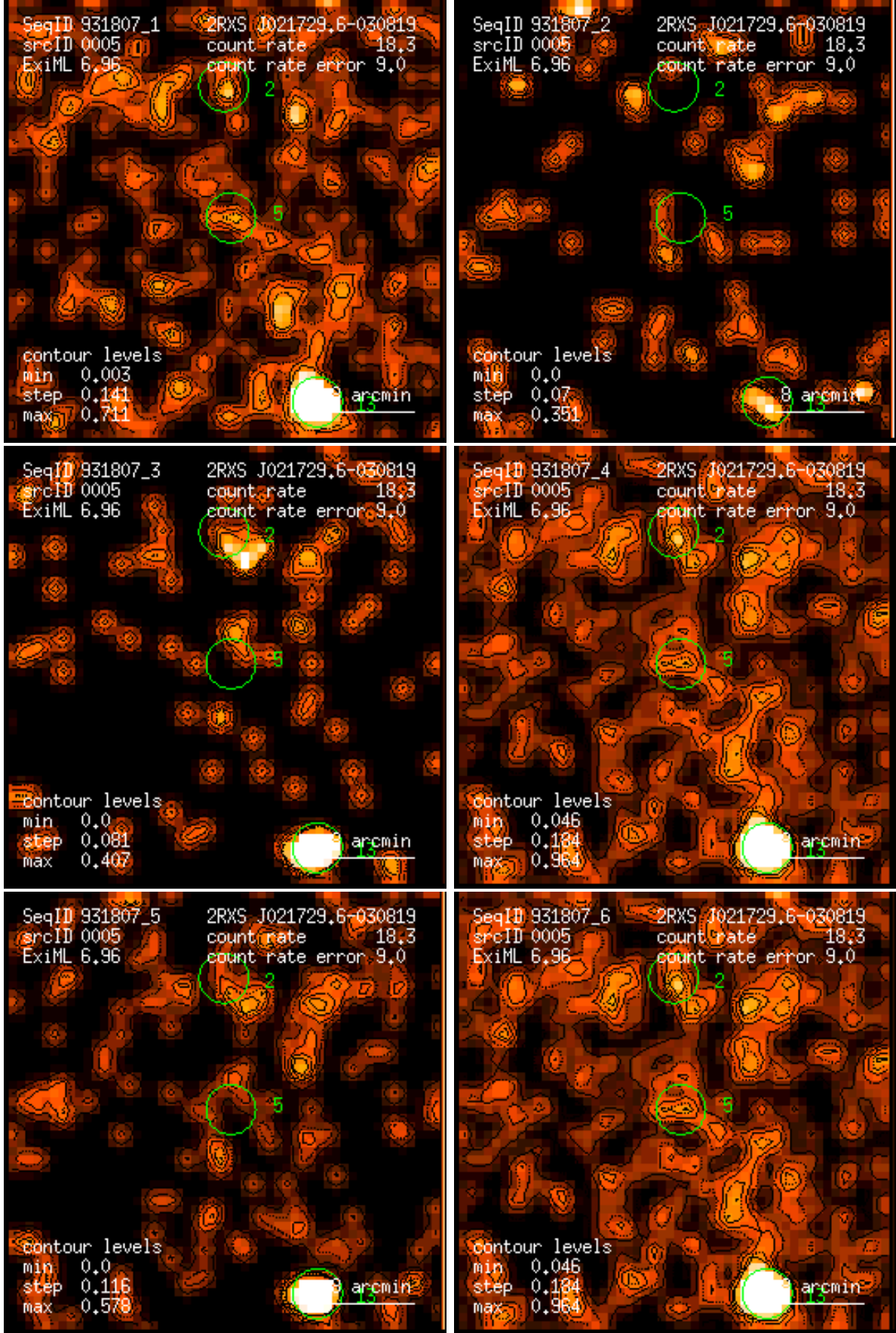
Figure 5: RASS 931807: detection 0005: band rate images, Gaussian filter: (1) PSPC channels 11 – 41, (2) 52 – 90, (3) 91 – 201, (4) 11 – 235, (5) 52 – 201, (6) 11 – 201. Broad band rates in counts/ks. Band rate contour levels in counts/ks/arcmin 2 .
