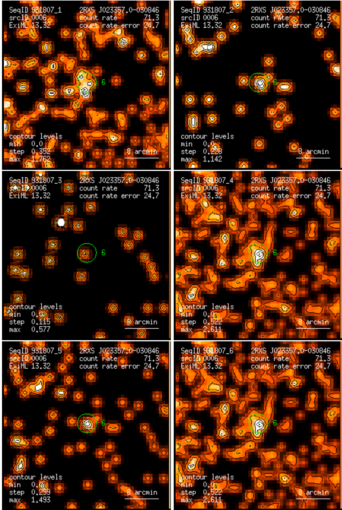
Figure 6: RASS 931807: detection 0006: band rate images, Gaussian filter: (1) PSPC channels 11 – 41, (2) 52 – 90, (3) 91 – 201, (4) 11 – 235, (5) 52 – 201, (6) 11 – 201. Broad band rates in counts/ks. Band rate contour levels in counts/ks/arcmin 2 .
