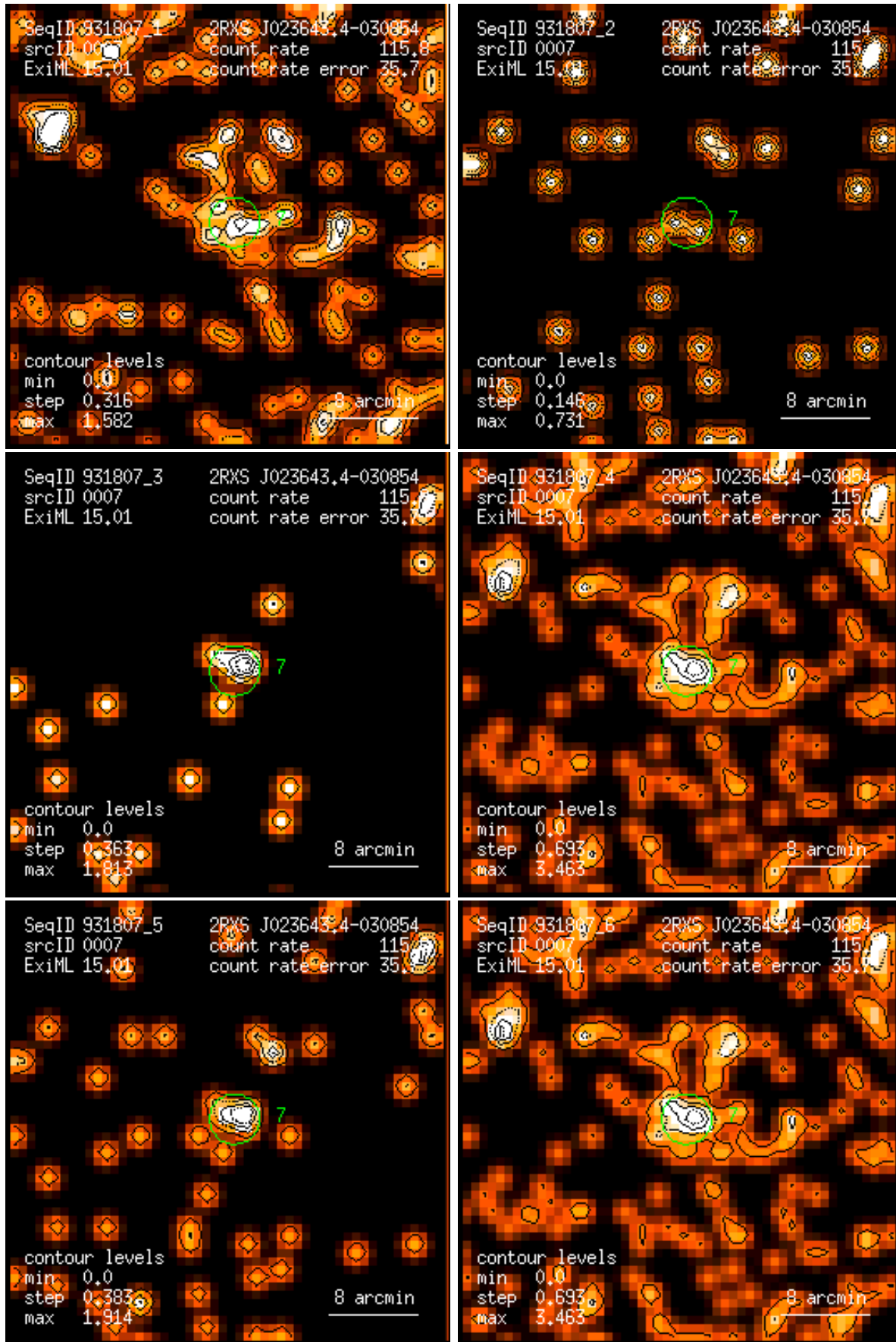
Figure 7: RASS 931807: detection 0007: band rate images, Gaussian filter: (1) PSPC channels 11 – 41, (2) 52 – 90, (3) 91 – 201, (4) 11 – 235, (5) 52 – 201, (6) 11 – 201. Broad band rates in counts/ks. Band rate contour levels in counts/ks/arcmin 2 .
