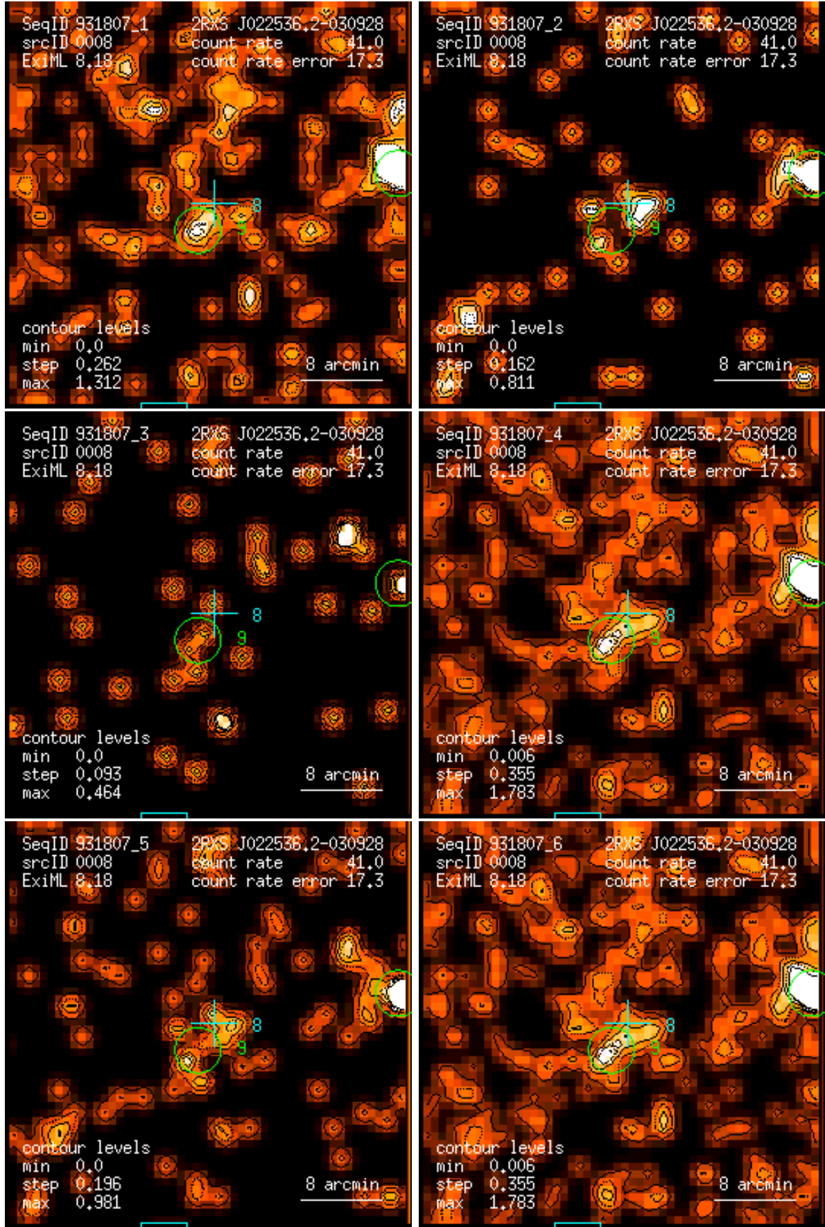
Figure 8: RASS 931807: detection 0008: band rate images, Gaussian filter: (1) PSPC channels 11 – 41, (2) 52 – 90, (3) 91 – 201, (4) 11 – 235, (5) 52 – 201, (6) 11 – 201. Broad band rates in counts/ks. Band rate contour levels in counts/ks/arcmin 2 .
