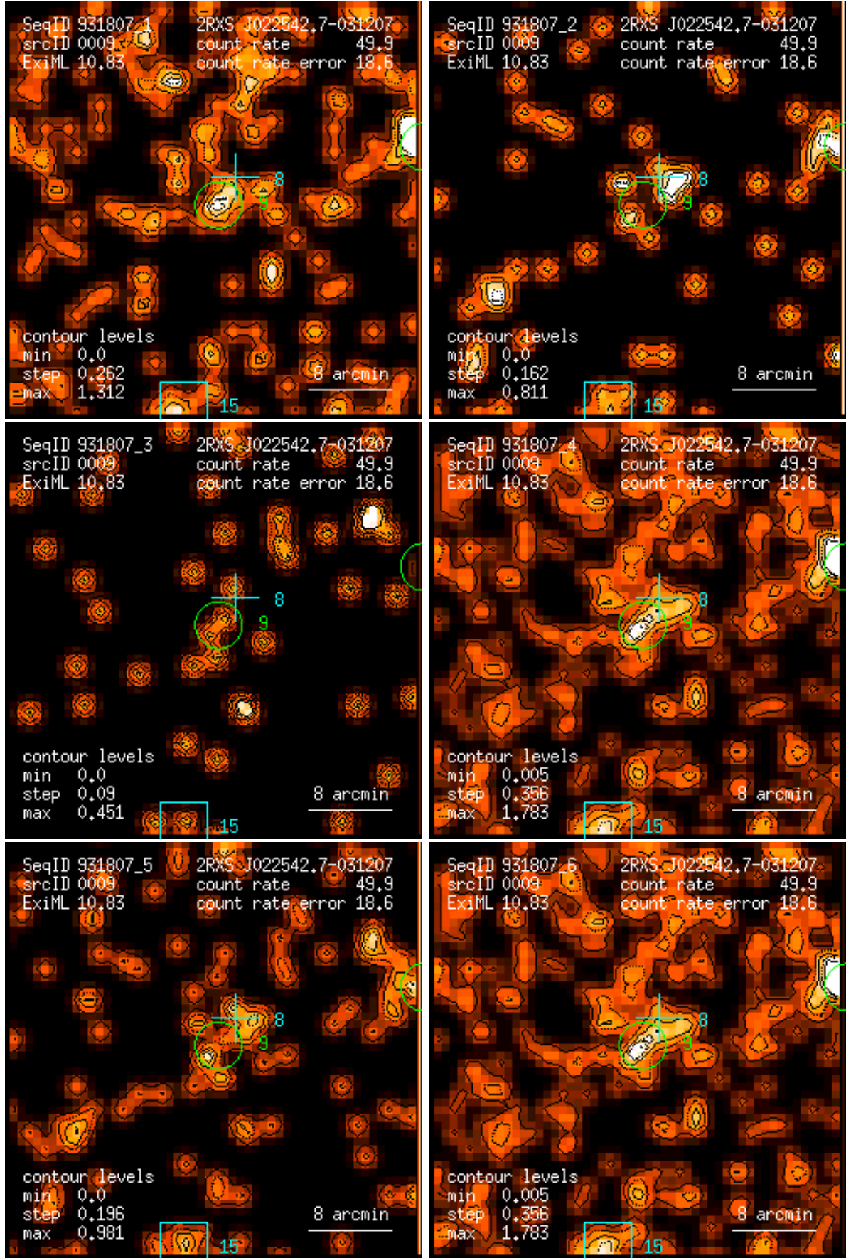
Figure 9: RASS 931807: detection 0009: band rate images, Gaussian filter: (1) PSPC channels 11 – 41, (2) 52 – 90, (3) 91 – 201, (4) 11 – 235, (5) 52 – 201, (6) 11 – 201. Broad band rates in counts/ks. Band rate contour levels in counts/ks/arcmin 2 .
