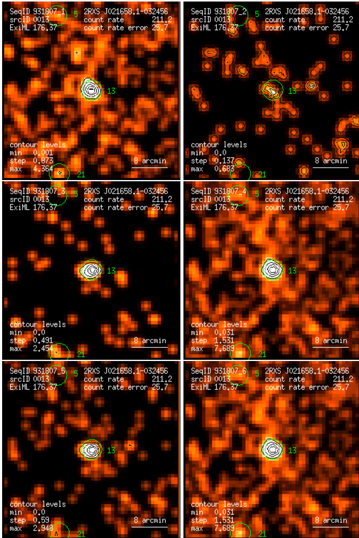
Figure 13: RASS 931807: detection 0013: band rate images, Gaussian filter: (1) PSPC channels 11 – 41, (2) 52 – 90, (3) 91 – 201, (4) 11 – 235, (5) 52 – 201, (6) 11 – 201. Broad band rates in counts/ks. Band rate contour levels in counts/ks/arcmin 2 .
