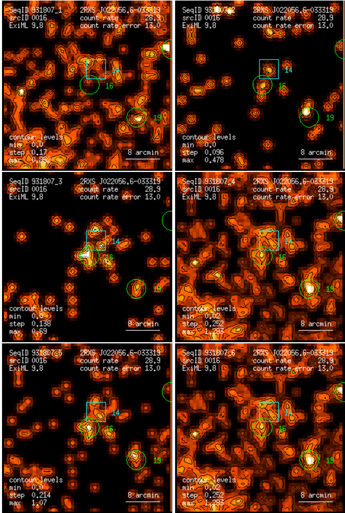
Figure 16: RASS 931807: detection 0016: band rate images, Gaussian filter: (1) PSPC channels 11 – 41, (2) 52 – 90, (3) 91 – 201, (4) 11 – 235, (5) 52 – 201, (6) 11 – 201. Broad band rates in counts/ks. Band rate contour levels in counts/ks/arcmin 2 .
