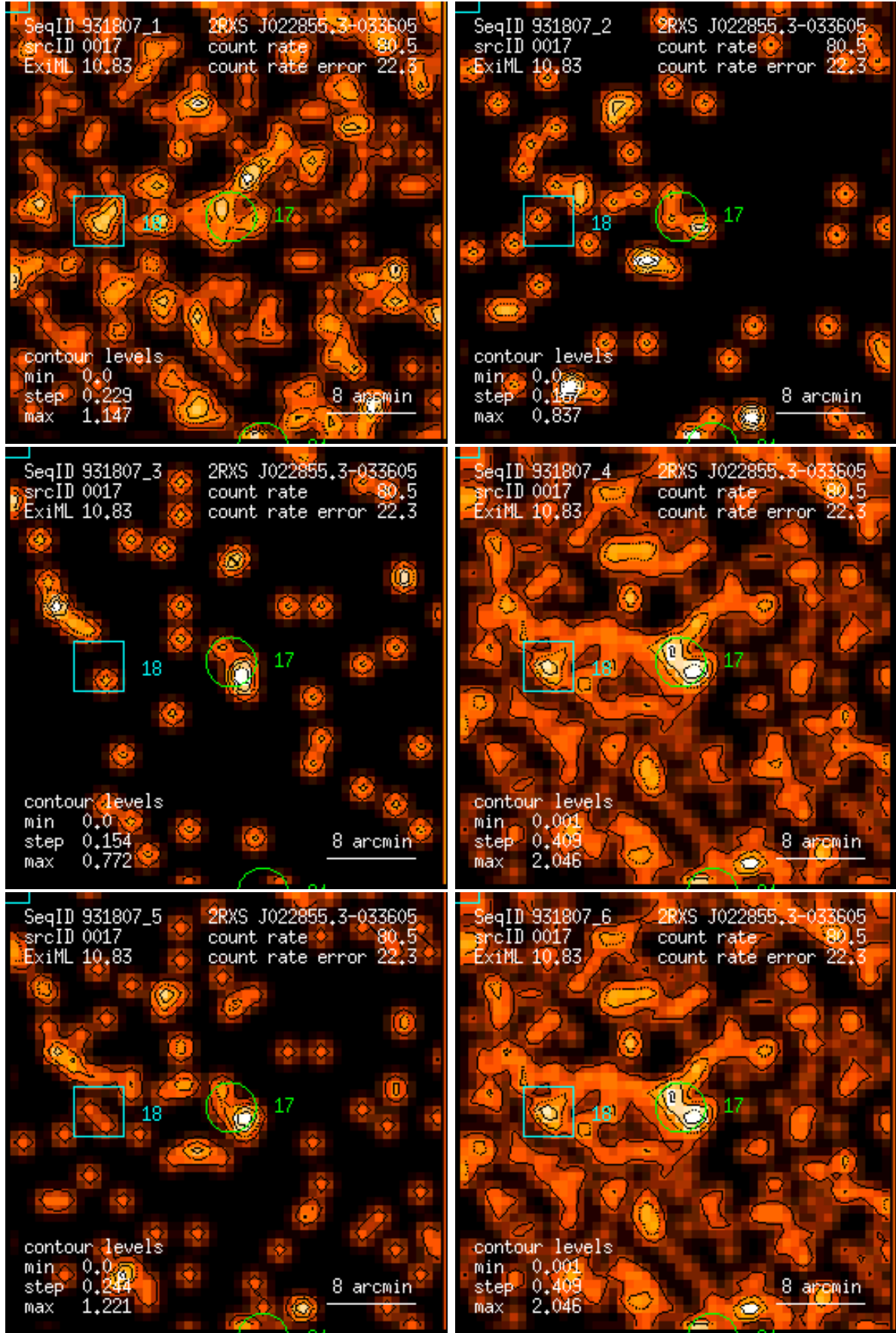
Figure 17: RASS 931807: detection 0017: band rate images, Gaussian filter: (1) PSPC channels 11 – 41, (2) 52 – 90, (3) 91 – 201, (4) 11 – 235, (5) 52 – 201, (6) 11 – 201. Broad band rates in counts/ks. Band rate contour levels in counts/ks/arcmin 2 .
