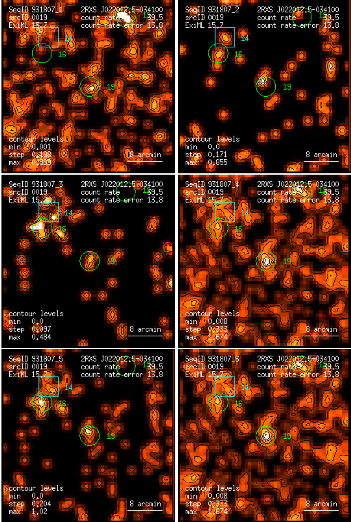
Figure 19: RASS 931807: detection 0019: band rate images, Gaussian filter: (1) PSPC channels 11 – 41, (2) 52 – 90, (3) 91 – 201, (4) 11 – 235, (5) 52 – 201, (6) 11 – 201. Broad band rates in counts/ks. Band rate contour levels in counts/ks/arcmin 2 .
