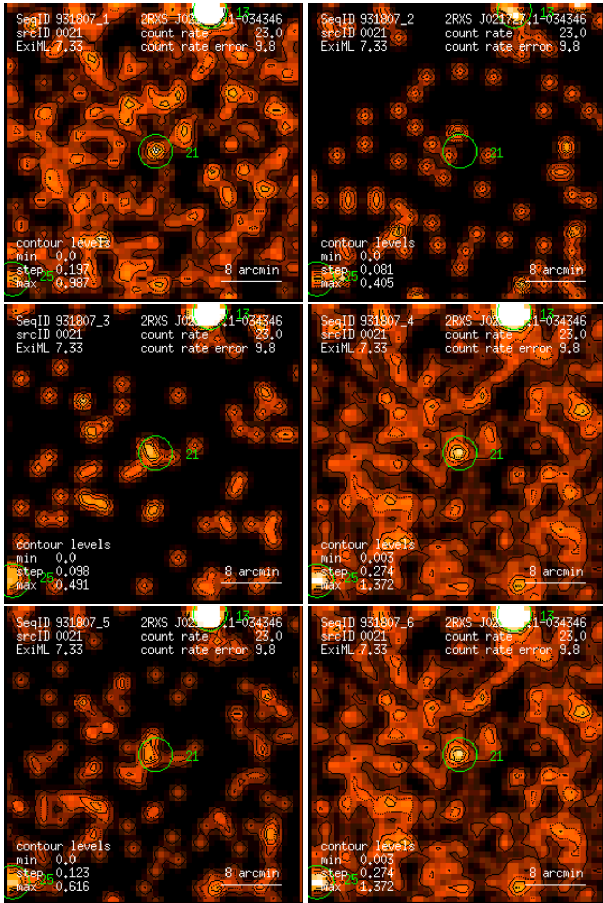
Figure 21: RASS 931807: detection 0021: band rate images, Gaussian filter: (1) PSPC channels 11 – 41, (2) 52 – 90, (3) 91 – 201, (4) 11 – 235, (5) 52 – 201, (6) 11 – 201. Broad band rates in counts/ks. Band rate contour levels in counts/ks/arcmin 2 .
