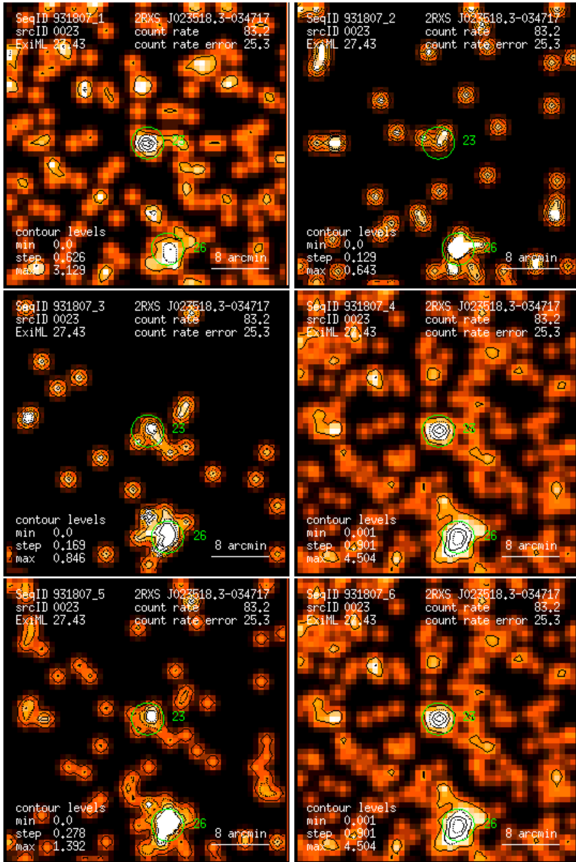
Figure 23: RASS 931807: detection 0023: band rate images, Gaussian filter: (1) PSPC channels 11 – 41, (2) 52 – 90, (3) 91 – 201, (4) 11 – 235, (5) 52 – 201, (6) 11 – 201. Broad band rates in counts/ks. Band rate contour levels in counts/ks/arcmin 2 .
