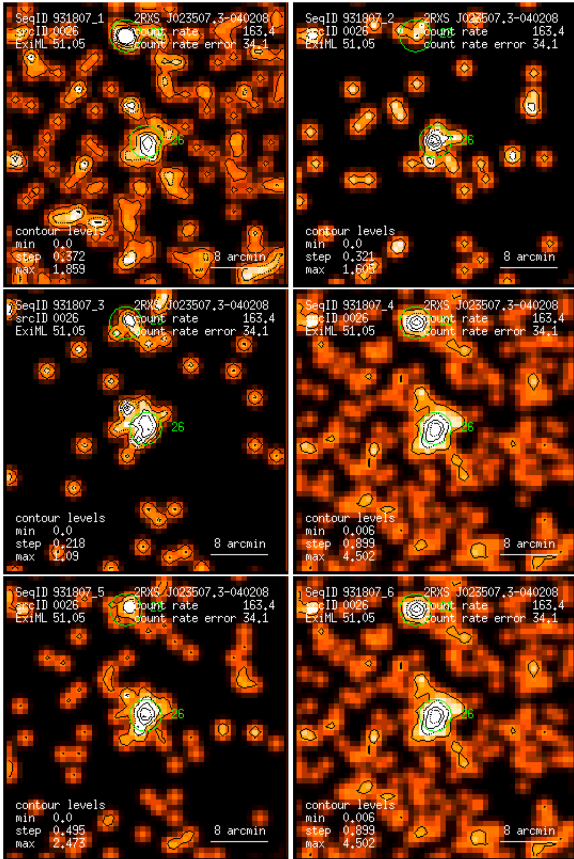
Figure 26: RASS 931807: detection 0026: band rate images, Gaussian filter: (1) PSPC channels 11 – 41, (2) 52 – 90, (3) 91 – 201, (4) 11 – 235, (5) 52 – 201, (6) 11 – 201. Broad band rates in counts/ks. Band rate contour levels in counts/ks/arcmin 2 .
