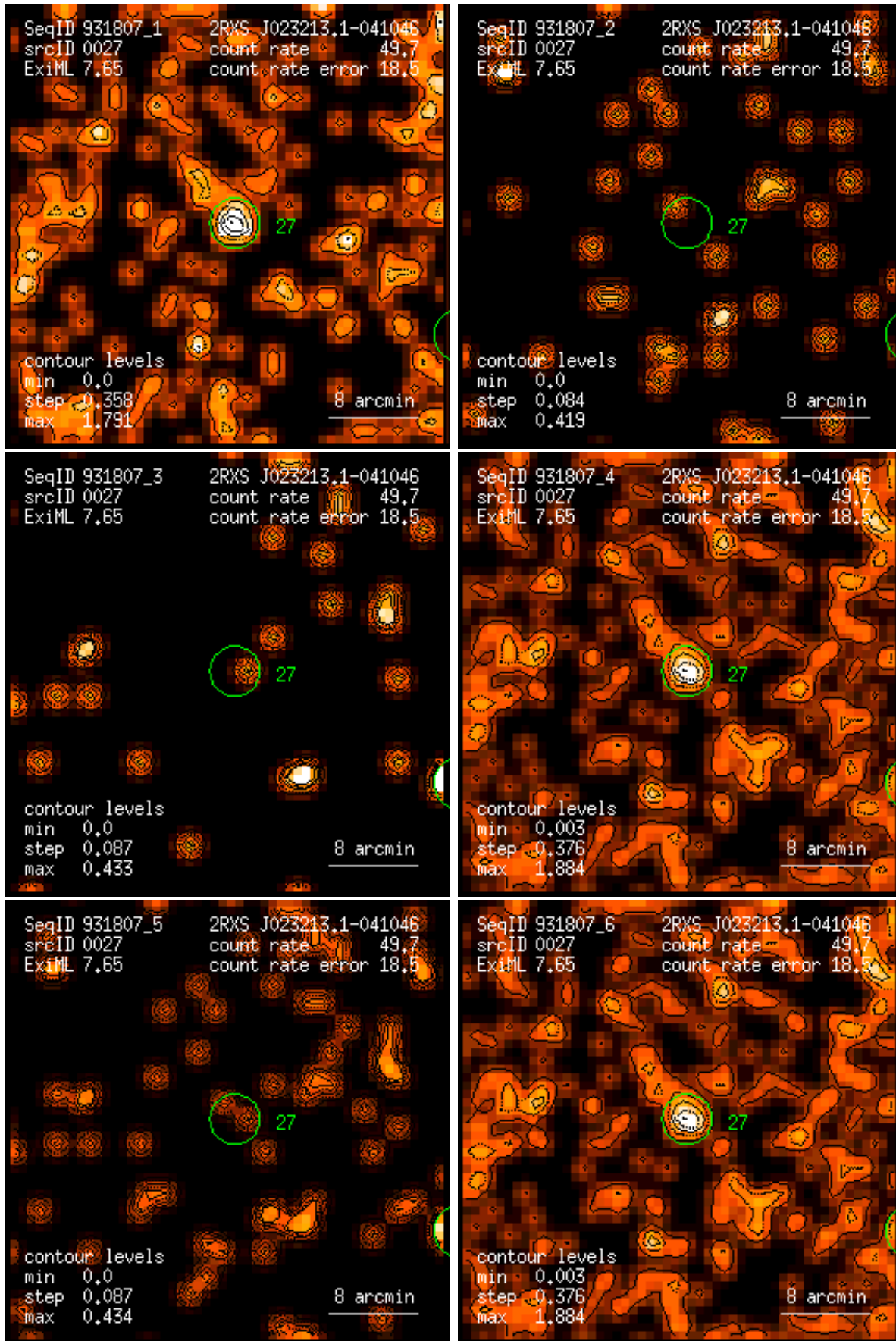
Figure 27: RASS 931807: detection 0027: band rate images, Gaussian filter: (1) PSPC channels 11 – 41, (2) 52 – 90, (3) 91 – 201, (4) 11 – 235, (5) 52 – 201, (6) 11 – 201. Broad band rates in counts/ks. Band rate contour levels in counts/ks/arcmin 2 .
