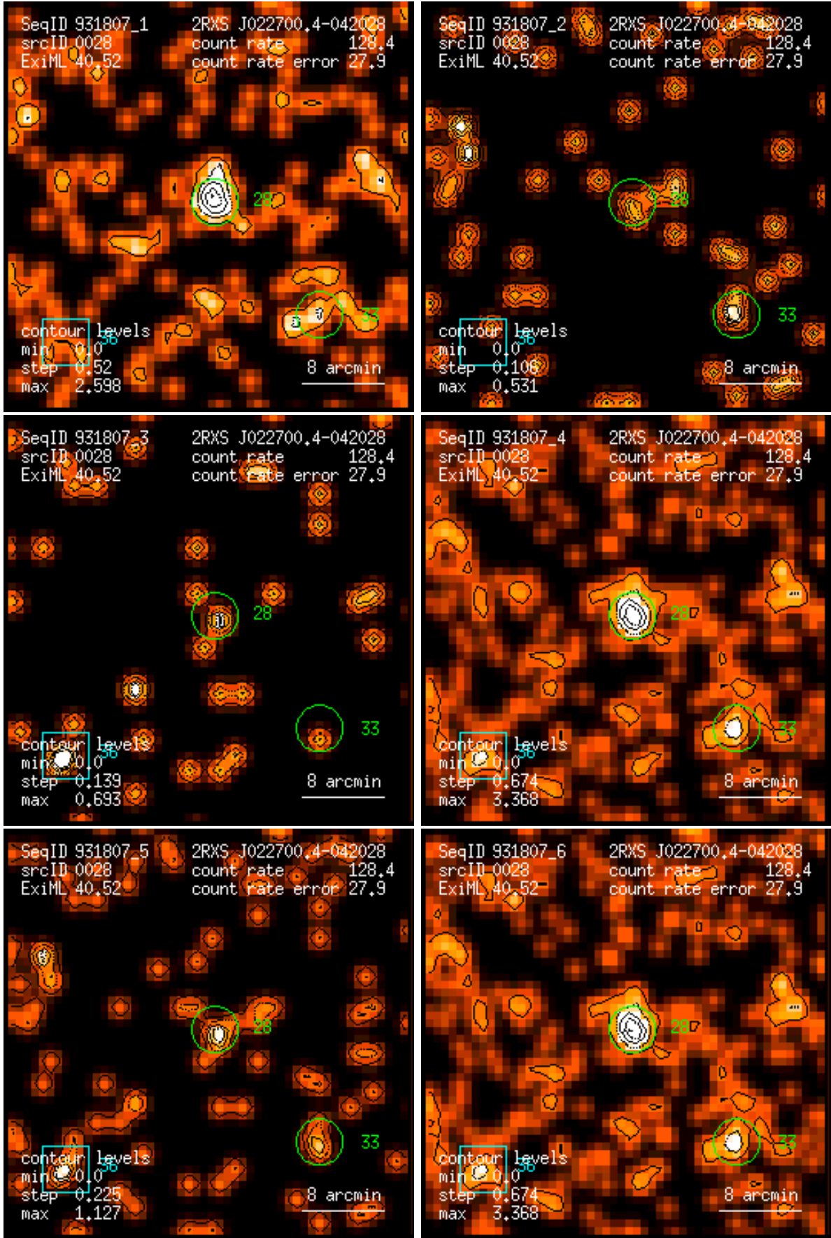
Figure 28: RASS 931807: detection 0028: band rate images, Gaussian filter: (1) PSPC channels 11 – 41, (2) 52 – 90, (3) 91 – 201, (4) 11 – 235, (5) 52 – 201, (6) 11 – 201. Broad band rates in counts/ks. Band rate contour levels in counts/ks/arcmin 2 .
