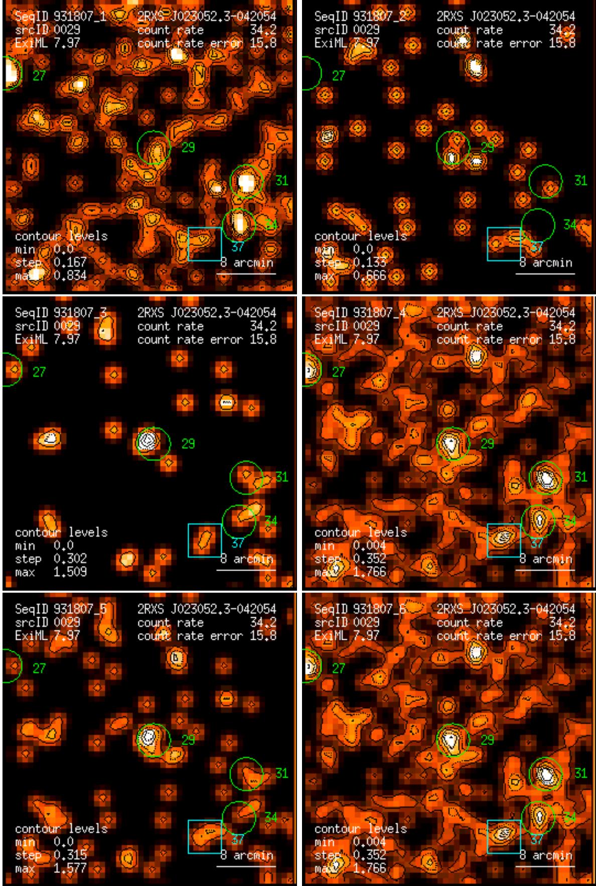
Figure 29: RASS 931807: detection 0029: band rate images, Gaussian filter: (1) PSPC channels 11 – 41, (2) 52 – 90, (3) 91 – 201, (4) 11 – 235, (5) 52 – 201, (6) 11 – 201. Broad band rates in counts/ks. Band rate contour levels in counts/ks/arcmin 2 .
