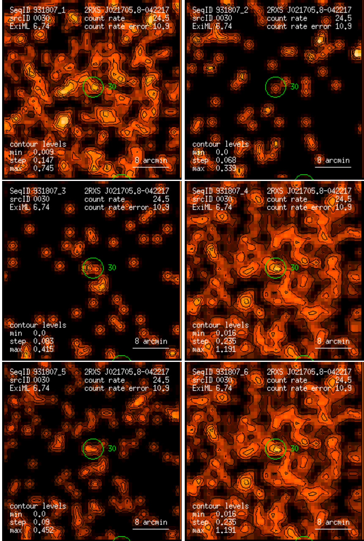
Figure 30: RASS 931807: detection 0030: band rate images, Gaussian filter: (1) PSPC channels 11 – 41, (2) 52 – 90, (3) 91 – 201, (4) 11 – 235, (5) 52 – 201, (6) 11 – 201. Broad band rates in counts/ks. Band rate contour levels in counts/ks/arcmin 2 .
