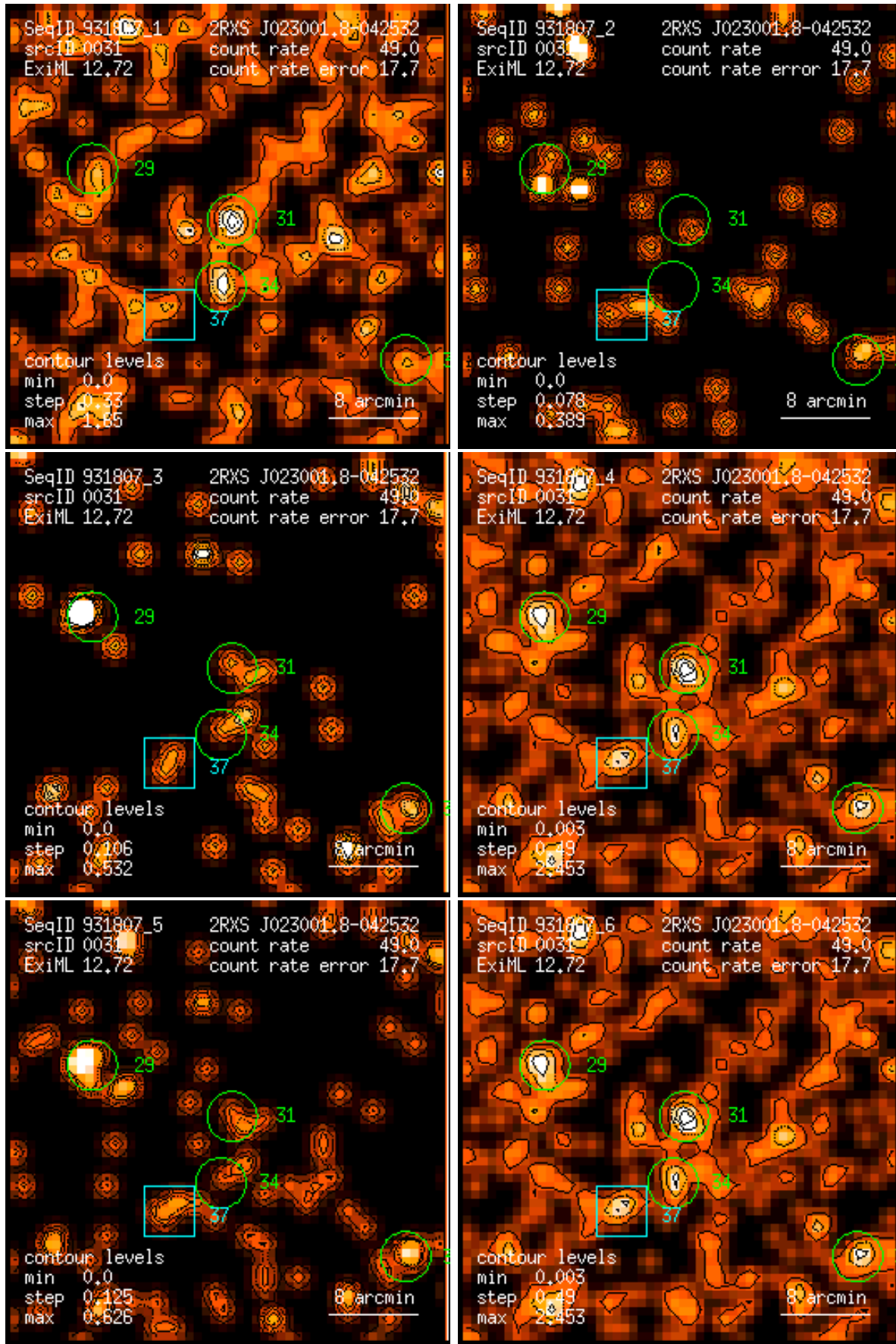
Figure 31: RASS 931807: detection 0031: band rate images, Gaussian filter: (1) PSPC channels 11 – 41, (2) 52 – 90, (3) 91 – 201, (4) 11 – 235, (5) 52 – 201, (6) 11 – 201. Broad band rates in counts/ks. Band rate contour levels in counts/ks/arcmin 2 .
