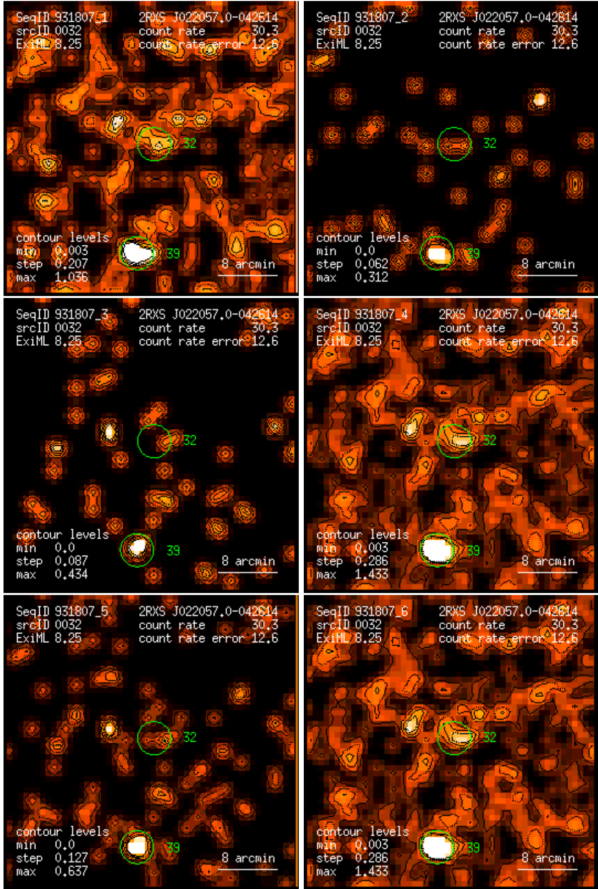
Figure 32: RASS 931807: detection 0032: band rate images, Gaussian filter: (1) PSPC channels 11 – 41, (2) 52 – 90, (3) 91 – 201, (4) 11 – 235, (5) 52 – 201, (6) 11 – 201. Broad band rates in counts/ks. Band rate contour levels in counts/ks/arcmin 2 .
