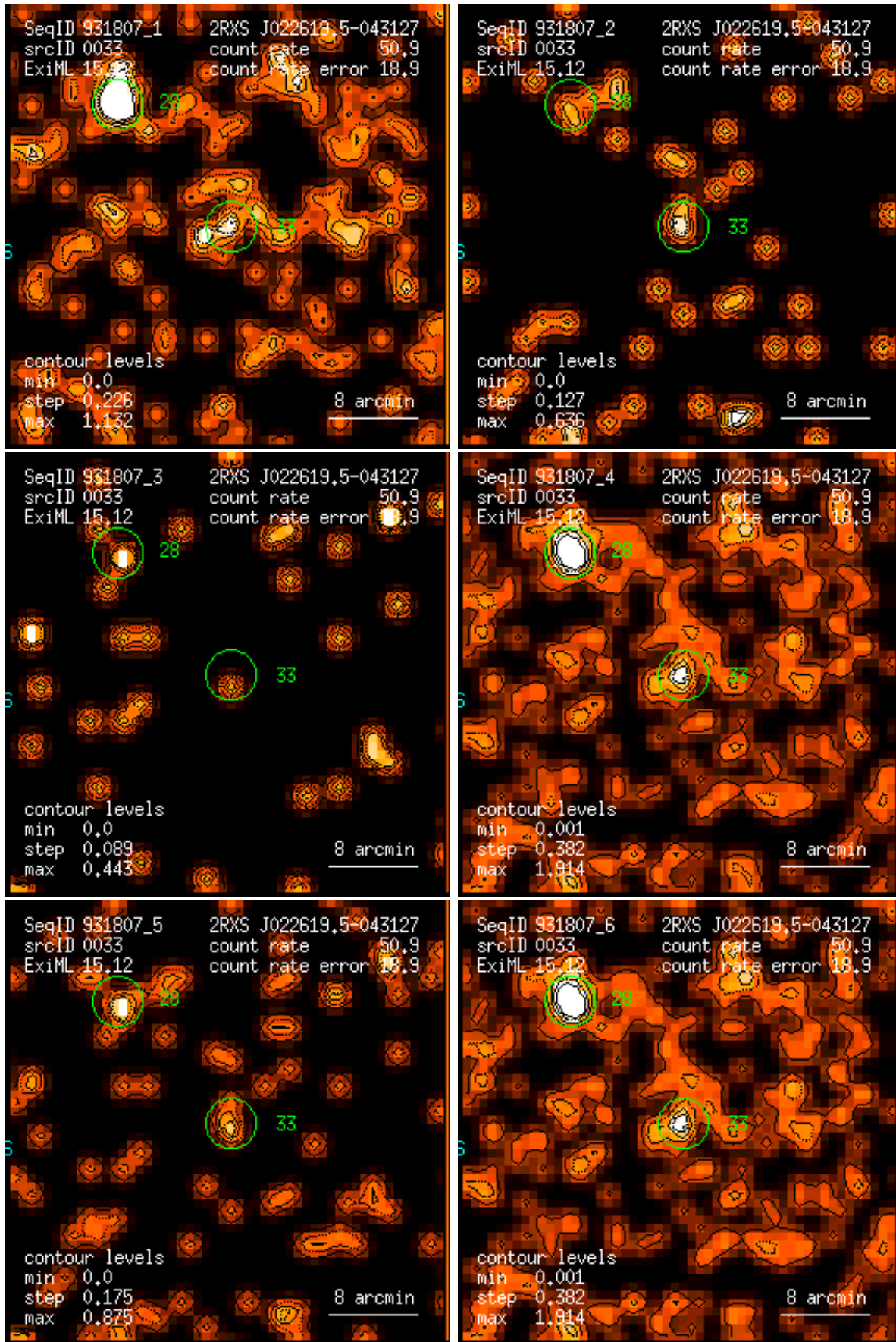
Figure 33: RASS 931807: detection 0033: band rate images, Gaussian filter: (1) PSPC channels 11 – 41, (2) 52 – 90, (3) 91 – 201, (4) 11 – 235, (5) 52 – 201, (6) 11 – 201. Broad band rates in counts/ks. Band rate contour levels in counts/ks/arcmin 2 .
