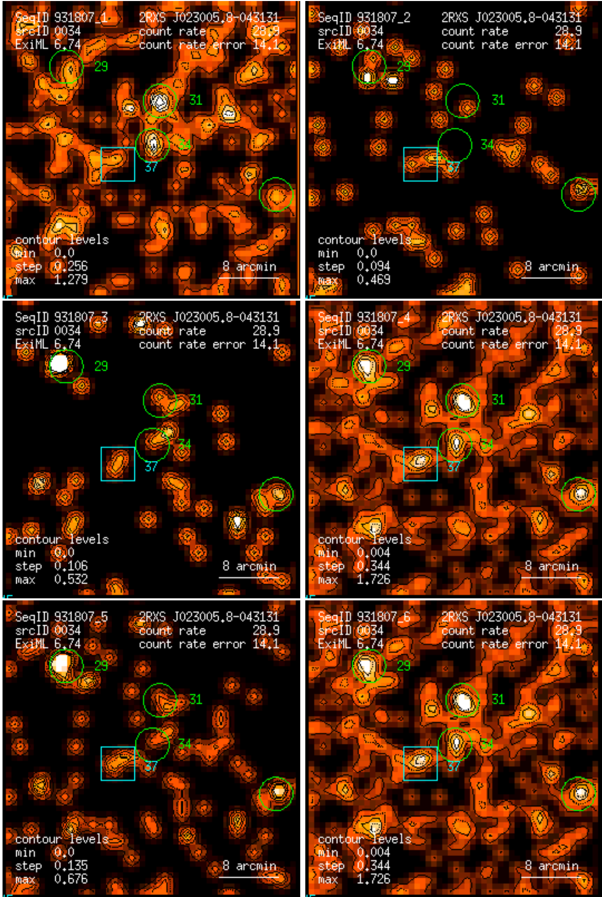
Figure 34: RASS 931807: detection 0034: band rate images, Gaussian filter: (1) PSPC channels 11 – 41, (2) 52 – 90, (3) 91 – 201, (4) 11 – 235, (5) 52 – 201, (6) 11 – 201. Broad band rates in counts/ks. Band rate contour levels in counts/ks/arcmin 2 .
