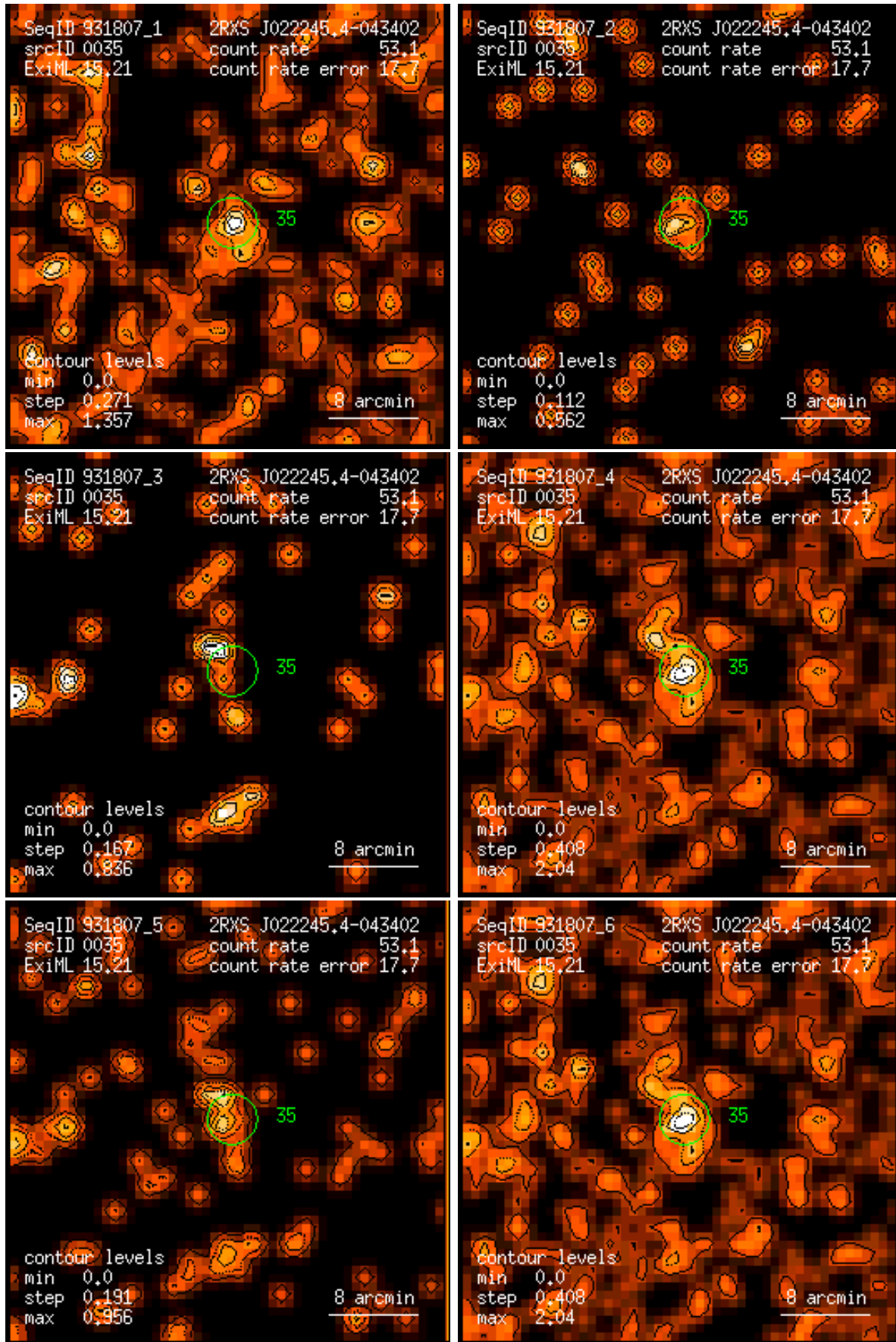
Figure 35: RASS 931807: detection 0035: band rate images, Gaussian filter: (1) PSPC channels 11 – 41, (2) 52 – 90, (3) 91 – 201, (4) 11 – 235, (5) 52 – 201, (6) 11 – 201. Broad band rates in counts/ks. Band rate contour levels in counts/ks/arcmin 2 .
