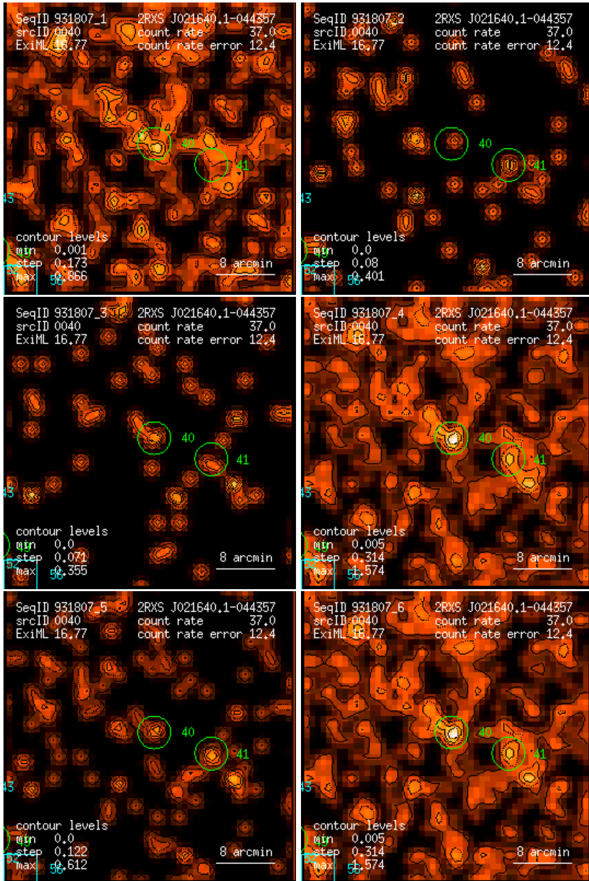
Figure 40: RASS 931807: detection 0040: band rate images, Gaussian filter: (1) PSPC channels 11 – 41, (2) 52 – 90, (3) 91 – 201, (4) 11 – 235, (5) 52 – 201, (6) 11 – 201. Broad band rates in counts/ks. Band rate contour levels in counts/ks/arcmin 2 .
