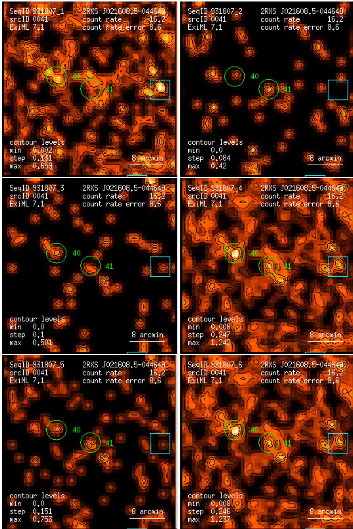
Figure 41: RASS 931807: detection 0041: band rate images, Gaussian filter: (1) PSPC channels 11 – 41, (2) 52 – 90, (3) 91 – 201, (4) 11 – 235, (5) 52 – 201, (6) 11 – 201. Broad band rates in counts/ks. Band rate contour levels in counts/ks/arcmin 2 .
