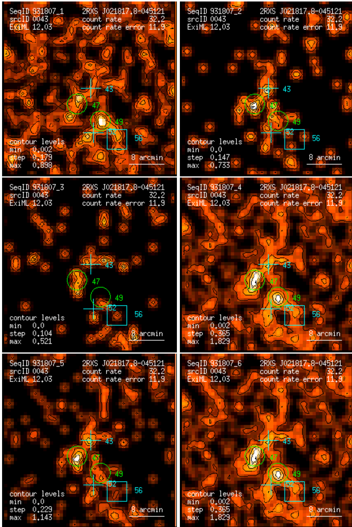
Figure 43: RASS 931807: detection 0043: band rate images, Gaussian filter: (1) PSPC channels 11 – 41, (2) 52 – 90, (3) 91 – 201, (4) 11 – 235, (5) 52 – 201, (6) 11 – 201. Broad band rates in counts/ks. Band rate contour levels in counts/ks/arcmin 2 .
