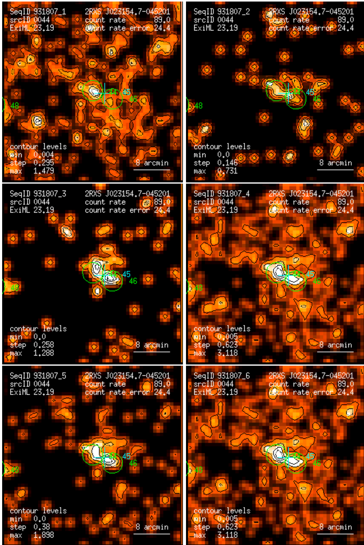
Figure 44: RASS 931807: detection 0044: band rate images, Gaussian filter: (1) PSPC channels 11 – 41, (2) 52 – 90, (3) 91 – 201, (4) 11 – 235, (5) 52 – 201, (6) 11 – 201. Broad band rates in counts/ks. Band rate contour levels in counts/ks/arcmin 2 .
