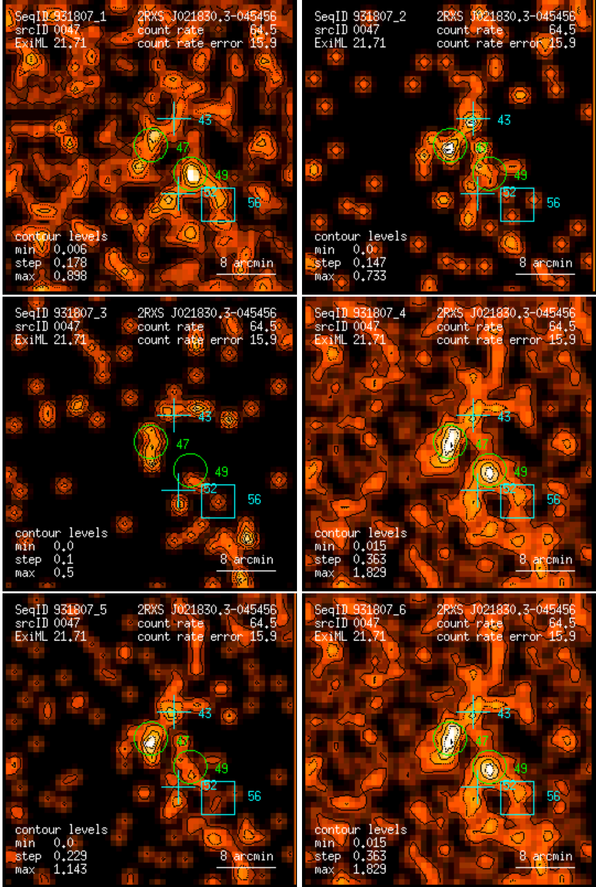
Figure 47: RASS 931807: detection 0047: band rate images, Gaussian filter: (1) PSPC channels 11 – 41, (2) 52 – 90, (3) 91 – 201, (4) 11 – 235, (5) 52 – 201, (6) 11 – 201. Broad band rates in counts/ks. Band rate contour levels in counts/ks/arcmin 2 .
