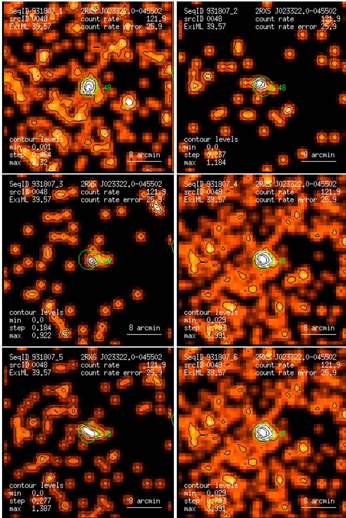
Figure 48: RASS 931807: detection 0048: band rate images, Gaussian filter: (1) PSPC channels 11 – 41, (2) 52 – 90, (3) 91 – 201, (4) 11 – 235, (5) 52 – 201, (6) 11 – 201. Broad band rates in counts/ks. Band rate contour levels in counts/ks/arcmin 2 .
