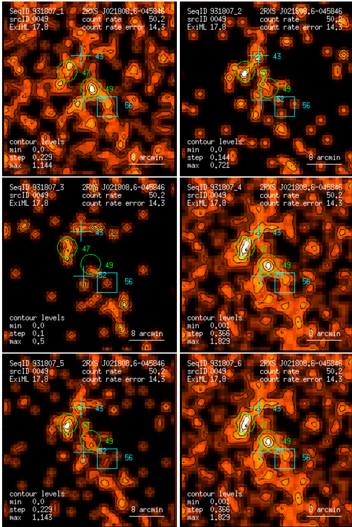
Figure 49: RASS 931807: detection 0049: band rate images, Gaussian filter: (1) PSPC channels 11 – 41, (2) 52 – 90, (3) 91 – 201, (4) 11 – 235, (5) 52 – 201, (6) 11 – 201. Broad band rates in counts/ks. Band rate contour levels in counts/ks/arcmin 2 .
