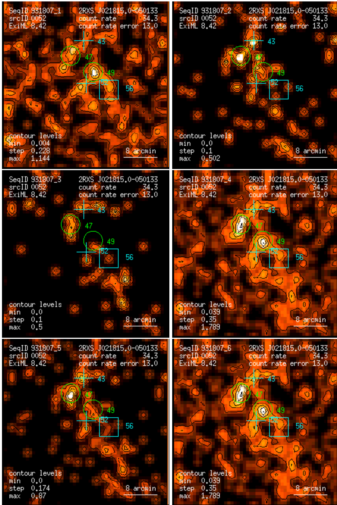
Figure 52: RASS 931807: detection 0052: band rate images, Gaussian filter: (1) PSPC channels 11 – 41, (2) 52 – 90, (3) 91 – 201, (4) 11 – 235, (5) 52 – 201, (6) 11 – 201. Broad band rates in counts/ks. Band rate contour levels in counts/ks/arcmin 2 .
