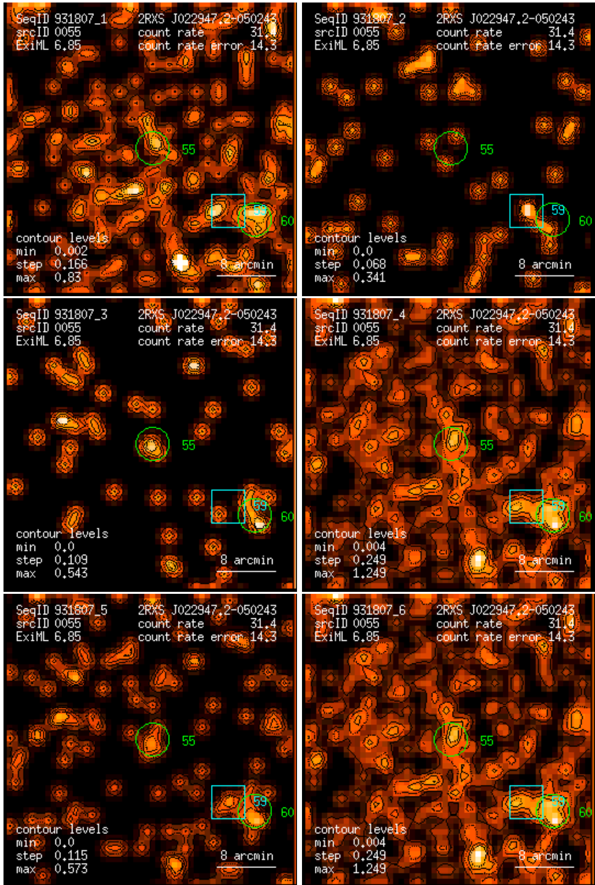
Figure 55: RASS 931807: detection 0055: band rate images, Gaussian filter: (1) PSPC channels 11 – 41, (2) 52 – 90, (3) 91 – 201, (4) 11 – 235, (5) 52 – 201, (6) 11 – 201. Broad band rates in counts/ks. Band rate contour levels in counts/ks/arcmin 2 .
