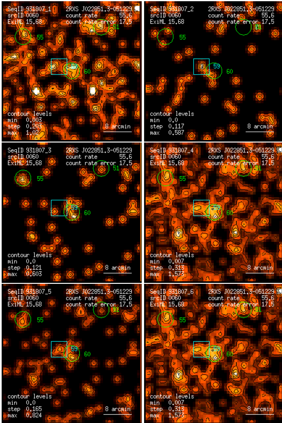
Figure 60: RASS 931807: detection 0060: band rate images, Gaussian filter: (1) PSPC channels 11 – 41, (2) 52 – 90, (3) 91 – 201, (4) 11 – 235, (5) 52 – 201, (6) 11 – 201. Broad band rates in counts/ks. Band rate contour levels in counts/ks/arcmin 2 .
