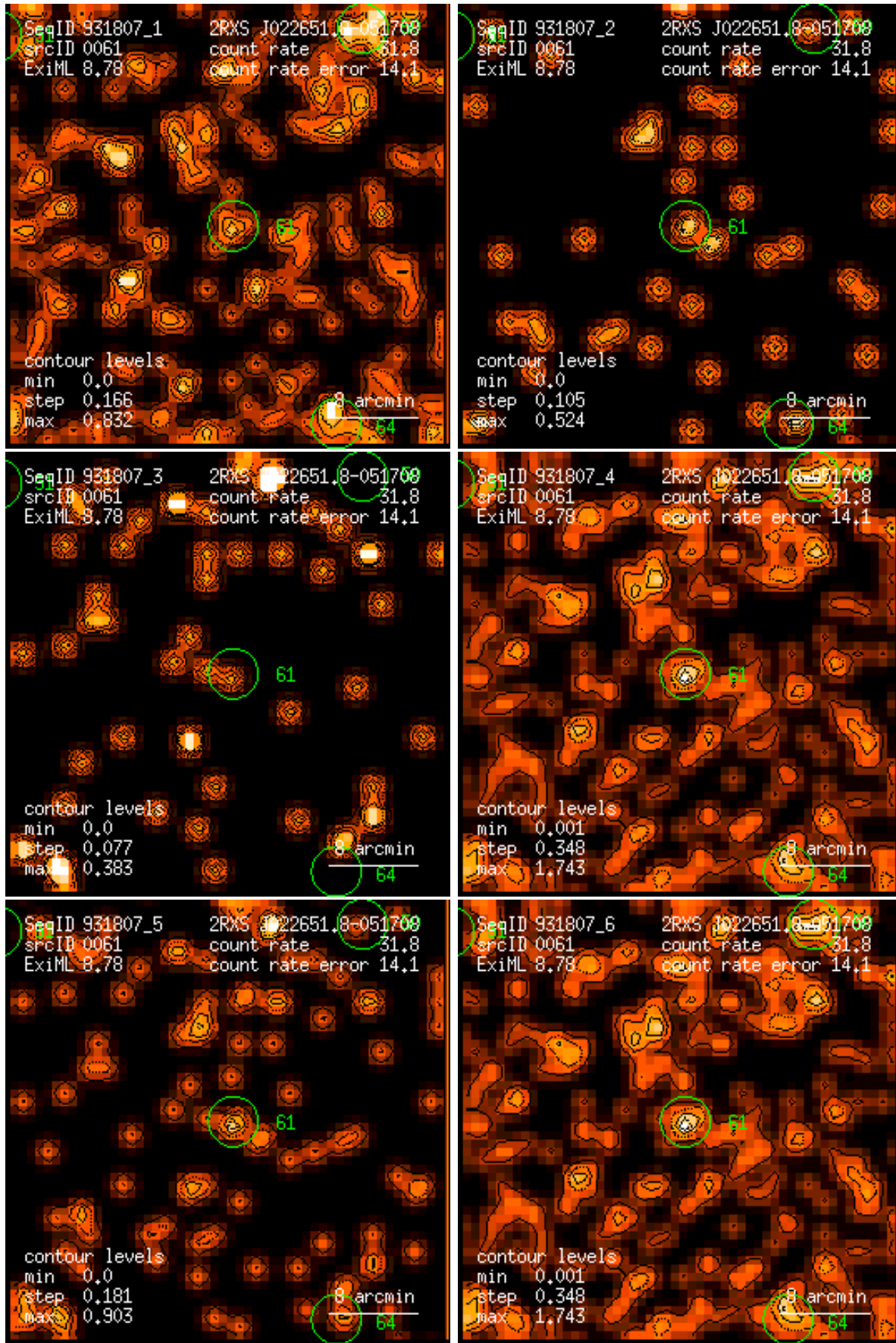
Figure 61: RASS 931807: detection 0061: band rate images, Gaussian filter: (1) PSPC channels 11 – 41, (2) 52 – 90, (3) 91 – 201, (4) 11 – 235, (5) 52 – 201, (6) 11 – 201. Broad band rates in counts/ks. Band rate contour levels in counts/ks/arcmin 2 .
