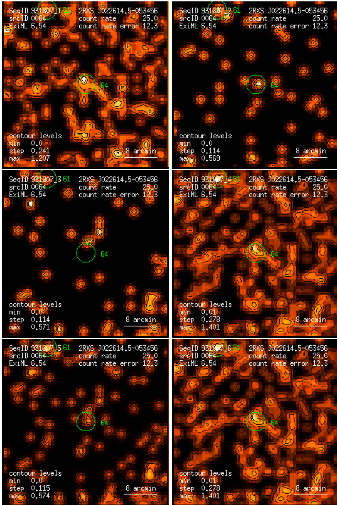
Figure 64: RASS 931807: detection 0064: band rate images, Gaussian filter: (1) PSPC channels 11 – 41, (2) 52 – 90, (3) 91 – 201, (4) 11 – 235, (5) 52 – 201, (6) 11 – 201. Broad band rates in counts/ks. Band rate contour levels in counts/ks/arcmin 2 .
