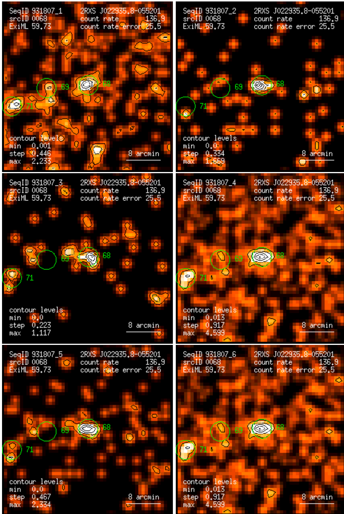
Figure 68: RASS 931807: detection 0068: band rate images, Gaussian filter: (1) PSPC channels 11 – 41, (2) 52 – 90, (3) 91 – 201, (4) 11 – 235, (5) 52 – 201, (6) 11 – 201. Broad band rates in counts/ks. Band rate contour levels in counts/ks/arcmin 2 .
