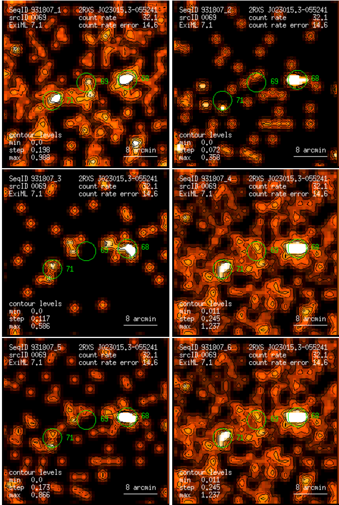
Figure 69: RASS 931807: detection 0069: band rate images, Gaussian filter: (1) PSPC channels 11 – 41, (2) 52 – 90, (3) 91 – 201, (4) 11 – 235, (5) 52 – 201, (6) 11 – 201. Broad band rates in counts/ks. Band rate contour levels in counts/ks/arcmin 2 .
