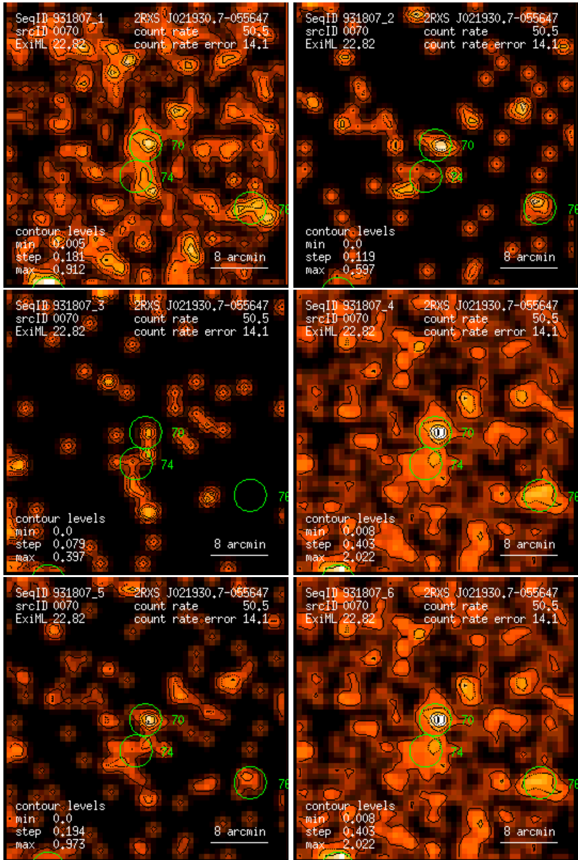
Figure 70: RASS 931807: detection 0070: band rate images, Gaussian filter: (1) PSPC channels 11 – 41, (2) 52 – 90, (3) 91 – 201, (4) 11 – 235, (5) 52 – 201, (6) 11 – 201. Broad band rates in counts/ks. Band rate contour levels in counts/ks/arcmin 2 .
