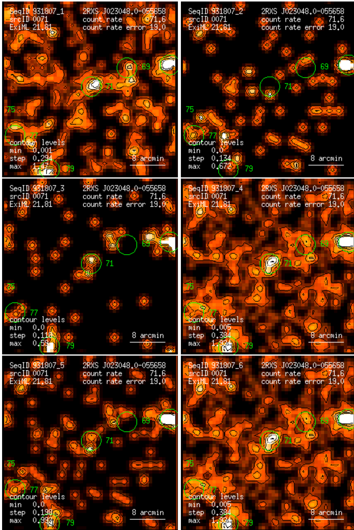
Figure 71: RASS 931807: detection 0071: band rate images, Gaussian filter: (1) PSPC channels 11 – 41, (2) 52 – 90, (3) 91 – 201, (4) 11 – 235, (5) 52 – 201, (6) 11 – 201. Broad band rates in counts/ks. Band rate contour levels in counts/ks/arcmin 2 .
