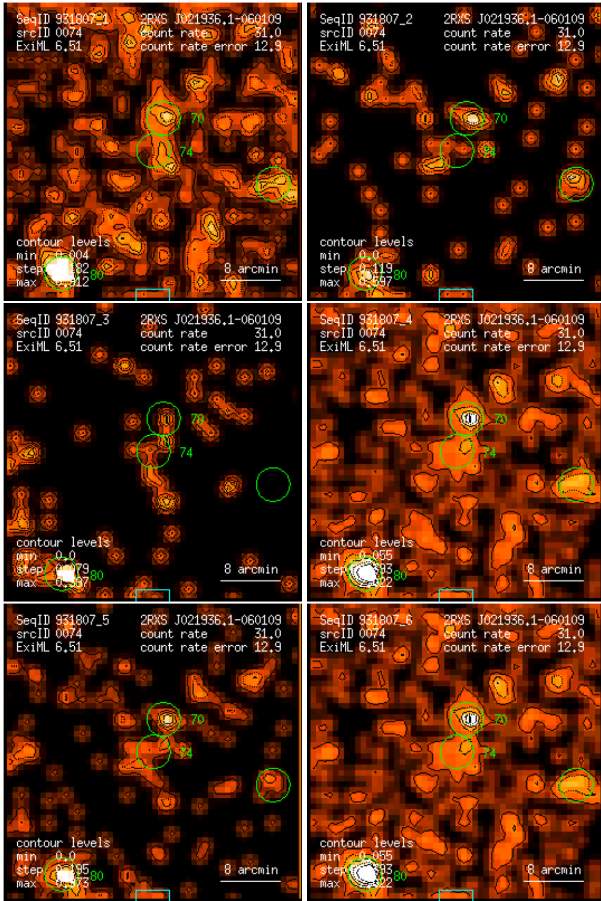
Figure 74: RASS 931807: detection 0074: band rate images, Gaussian filter: (1) PSPC channels 11 – 41, (2) 52 – 90, (3) 91 – 201, (4) 11 – 235, (5) 52 – 201, (6) 11 – 201. Broad band rates in counts/ks. Band rate contour levels in counts/ks/arcmin 2 .
