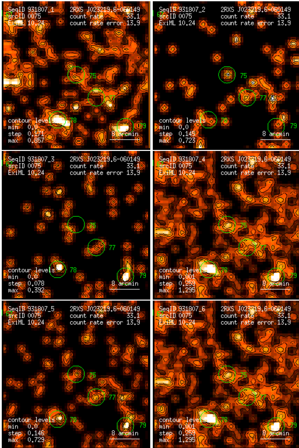
Figure 75: RASS 931807: detection 0075: band rate images, Gaussian filter: (1) PSPC channels 11 – 41, (2) 52 – 90, (3) 91 – 201, (4) 11 – 235, (5) 52 – 201, (6) 11 – 201. Broad band rates in counts/ks. Band rate contour levels in counts/ks/arcmin 2 .
