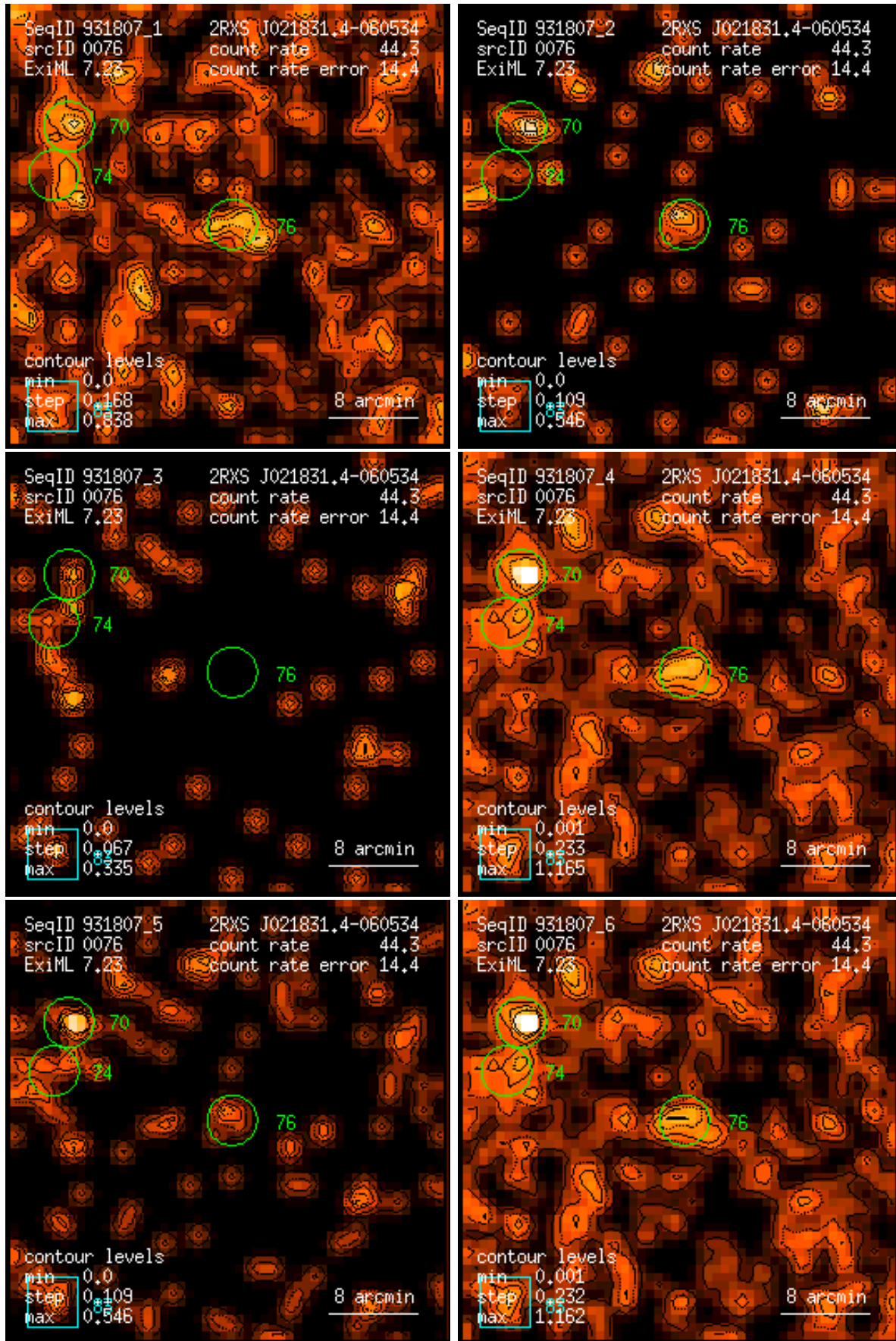
Figure 76: RASS 931807: detection 0076: band rate images, Gaussian filter: (1) PSPC channels 11 – 41, (2) 52 – 90, (3) 91 – 201, (4) 11 – 235, (5) 52 – 201, (6) 11 – 201. Broad band rates in counts/ks. Band rate contour levels in counts/ks/arcmin 2 .
