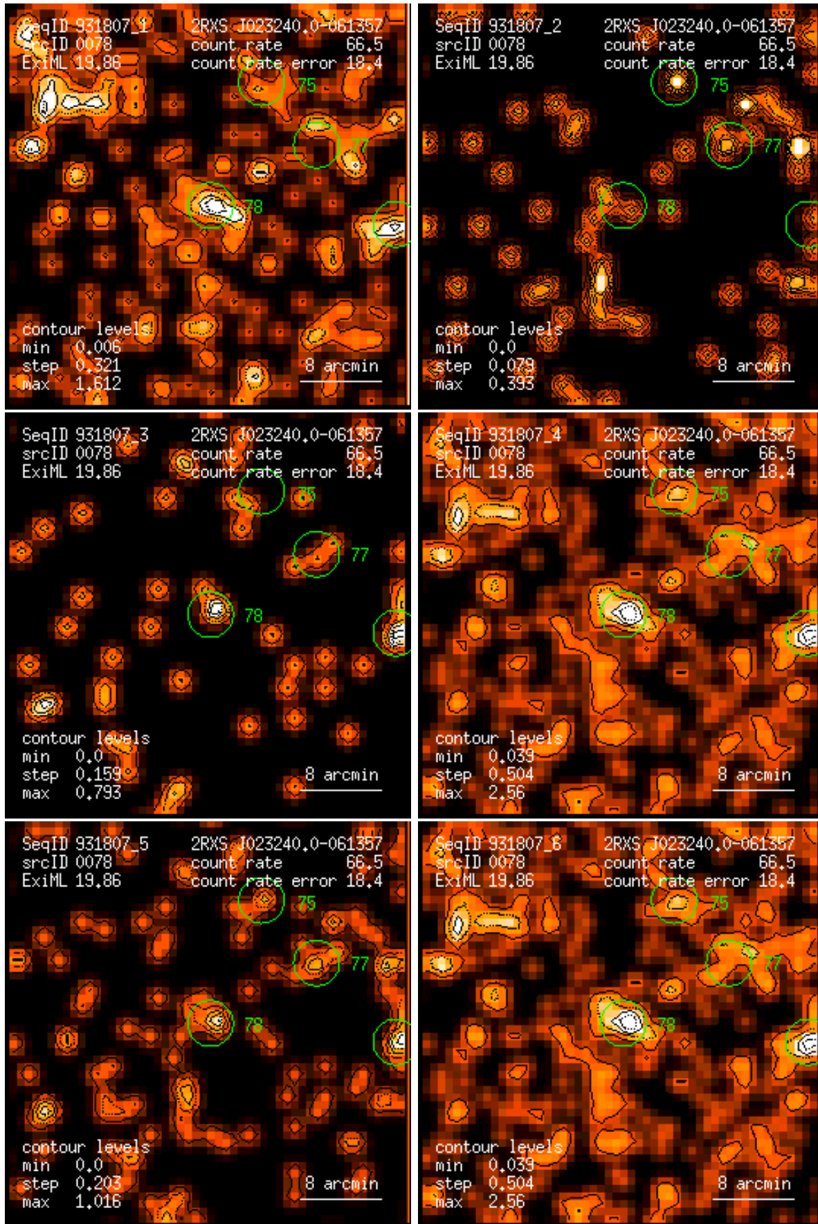
Figure 78: RASS 931807: detection 0078: band rate images, Gaussian filter: (1) PSPC channels 11 – 41, (2) 52 – 90, (3) 91 – 201, (4) 11 – 235, (5) 52 – 201, (6) 11 – 201. Broad band rates in counts/ks. Band rate contour levels in counts/ks/arcmin 2 .
