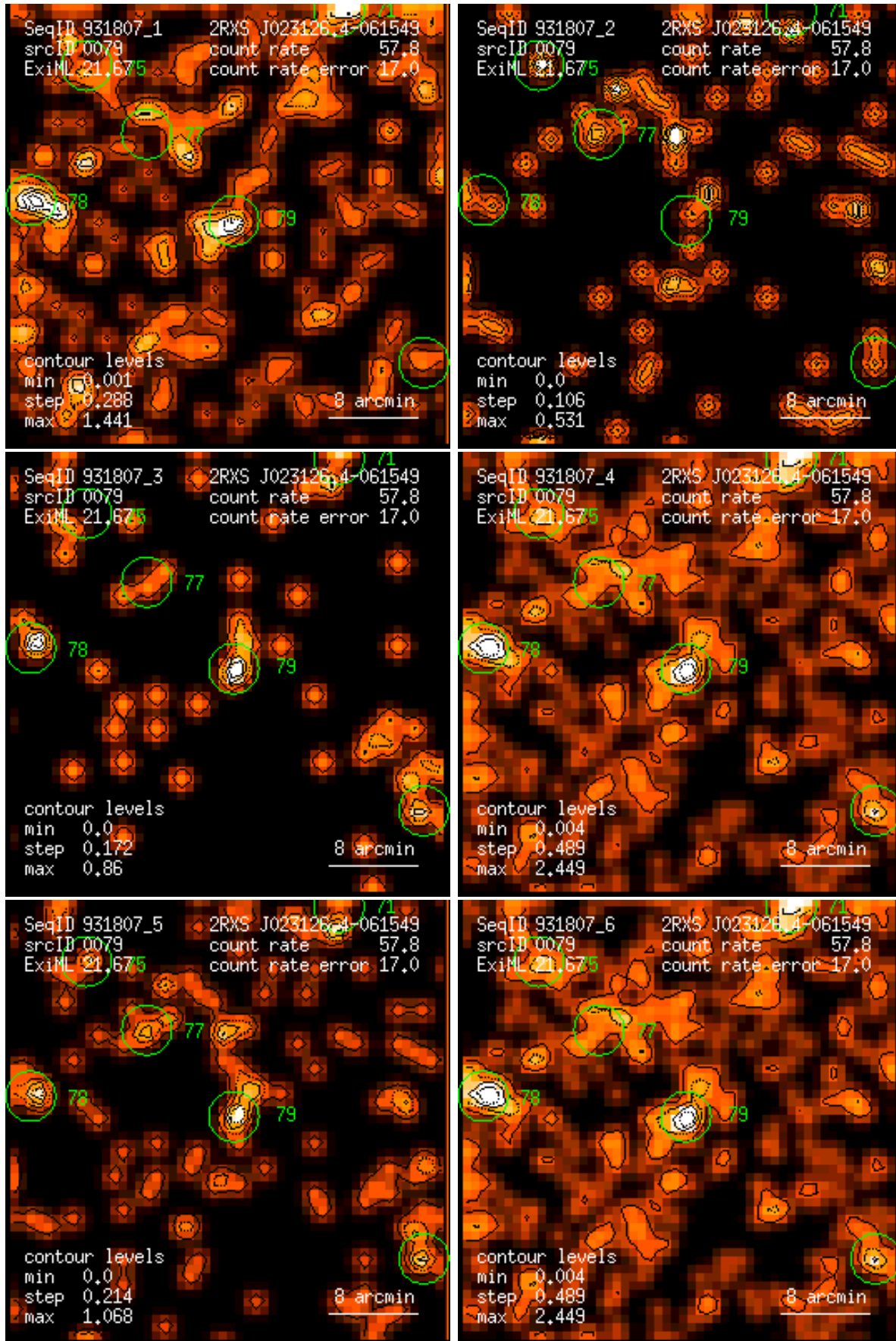
Figure 79: RASS 931807: detection 0079: band rate images, Gaussian filter: (1) PSPC channels 11 – 41, (2) 52 – 90, (3) 91 – 201, (4) 11 – 235, (5) 52 – 201, (6) 11 – 201. Broad band rates in counts/ks. Band rate contour levels in counts/ks/arcmin 2 .
