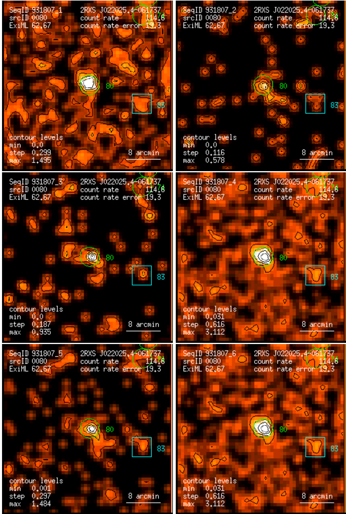
Figure 80: RASS 931807: detection 0080: band rate images, Gaussian filter: (1) PSPC channels 11 – 41, (2) 52 – 90, (3) 91 – 201, (4) 11 – 235, (5) 52 – 201, (6) 11 – 201. Broad band rates in counts/ks. Band rate contour levels in counts/ks/arcmin 2 .
