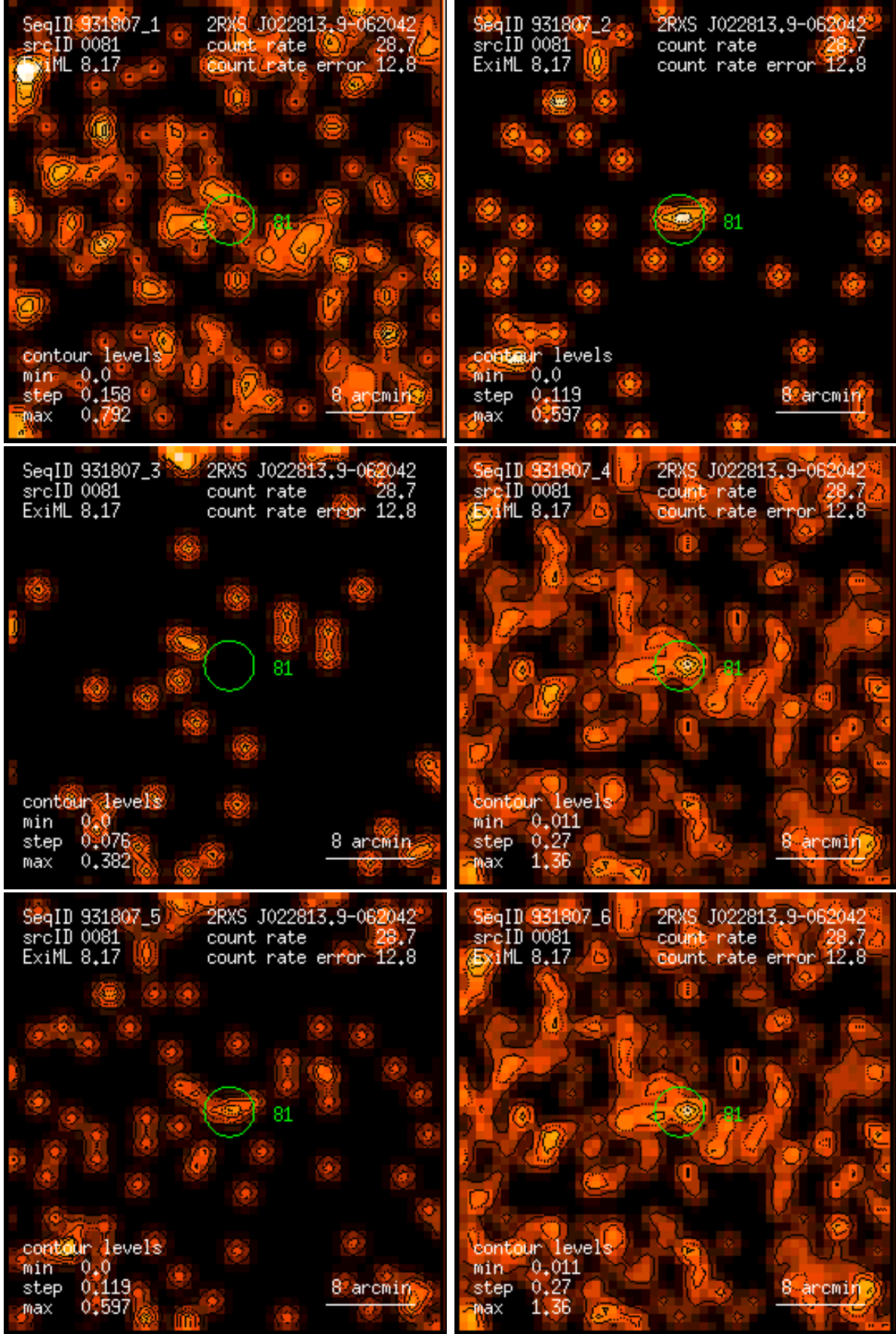
Figure 81: RASS 931807: detection 0081: band rate images, Gaussian filter: (1) PSPC channels 11 – 41, (2) 52 – 90, (3) 91 – 201, (4) 11 – 235, (5) 52 – 201, (6) 11 – 201. Broad band rates in counts/ks. Band rate contour levels in counts/ks/arcmin 2 .
