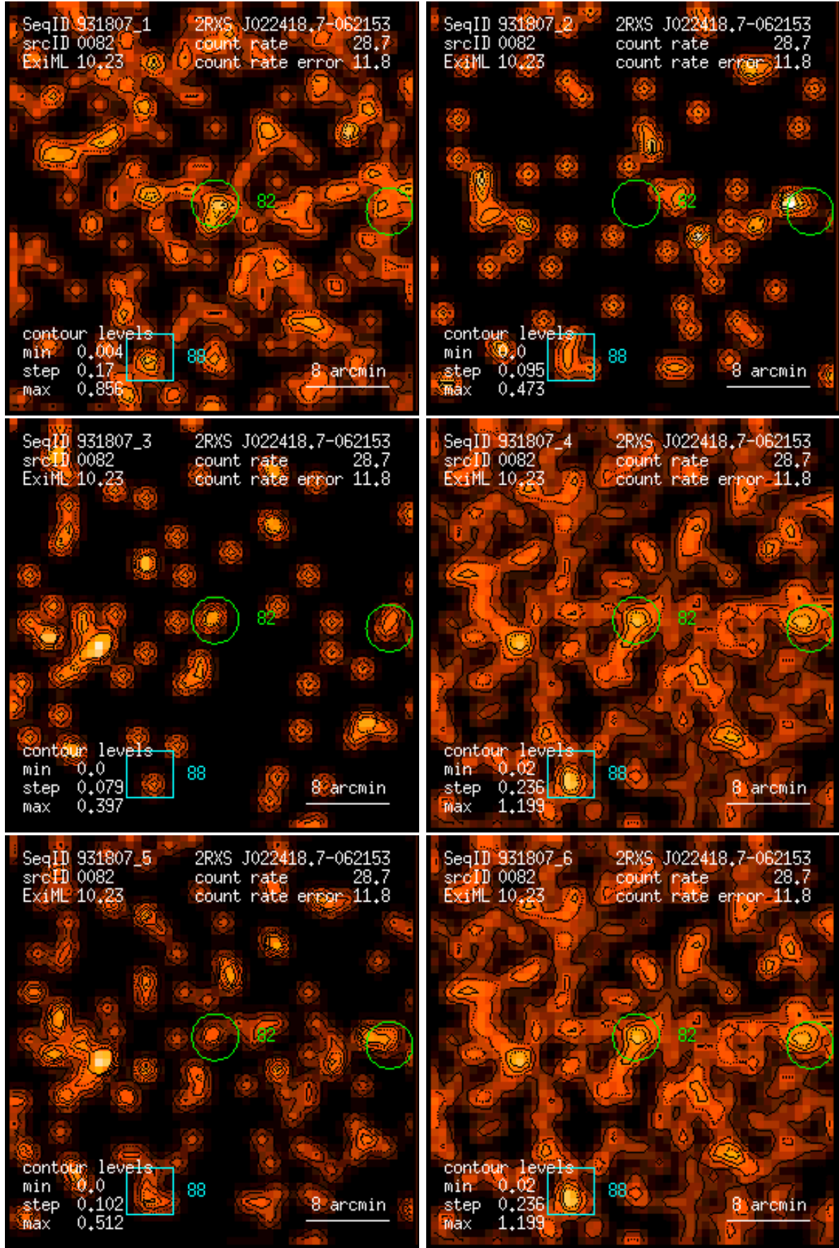
Figure 82: RASS 931807: detection 0082: band rate images, Gaussian filter: (1) PSPC channels 11 – 41, (2) 52 – 90, (3) 91 – 201, (4) 11 – 235, (5) 52 – 201, (6) 11 – 201. Broad band rates in counts/ks. Band rate contour levels in counts/ks/arcmin 2 .
