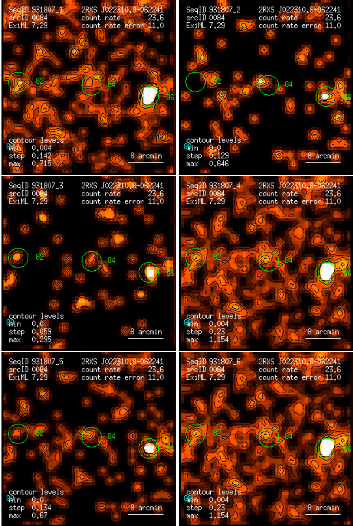
Figure 84: RASS 931807: detection 0084: band rate images, Gaussian filter: (1) PSPC channels 11 – 41, (2) 52 – 90, (3) 91 – 201, (4) 11 – 235, (5) 52 – 201, (6) 11 – 201. Broad band rates in counts/ks. Band rate contour levels in counts/ks/arcmin 2 .
