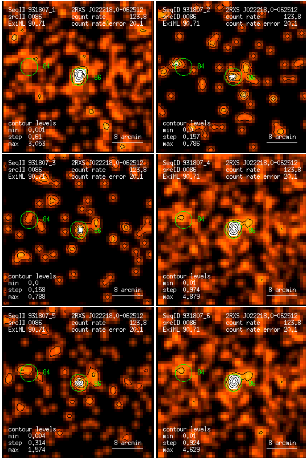
Figure 86: RASS 931807: detection 0086: band rate images, Gaussian filter: (1) PSPC channels 11 – 41, (2) 52 – 90, (3) 91 – 201, (4) 11 – 235, (5) 52 – 201, (6) 11 – 201. Broad band rates in counts/ks. Band rate contour levels in counts/ks/arcmin 2 .
